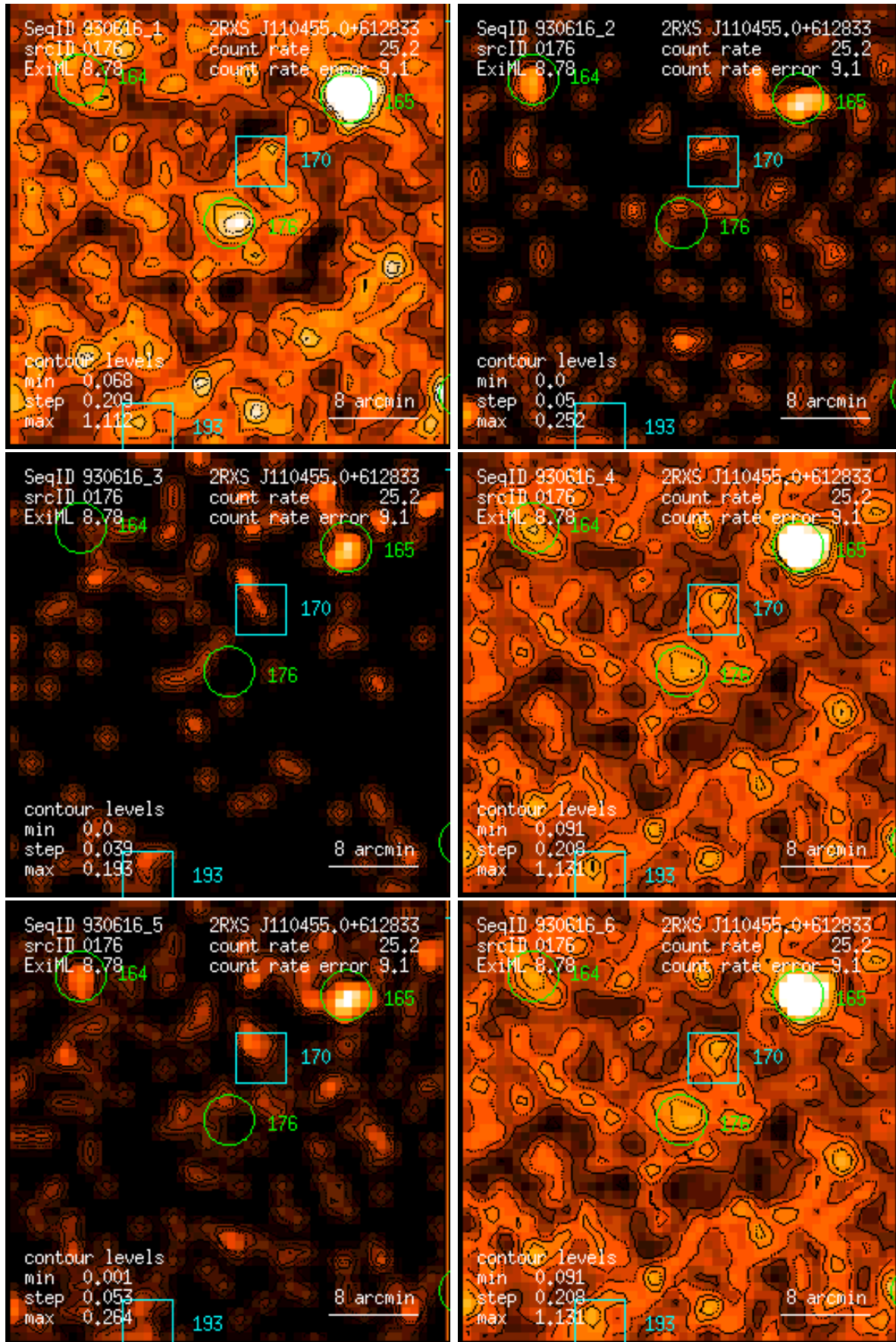
Figure 176: RASS 930616: detection 0176: band rate images, Gaussian filter: (1) PSPC channels 11 – 41, (2) 52 – 90, (3) 91 – 201, (4) 11 – 235, (5) 52 – 201, (6) 11 – 201. Broad band rates in counts/ks. Band rate contour levels in counts/ks/arcmin 2 .
