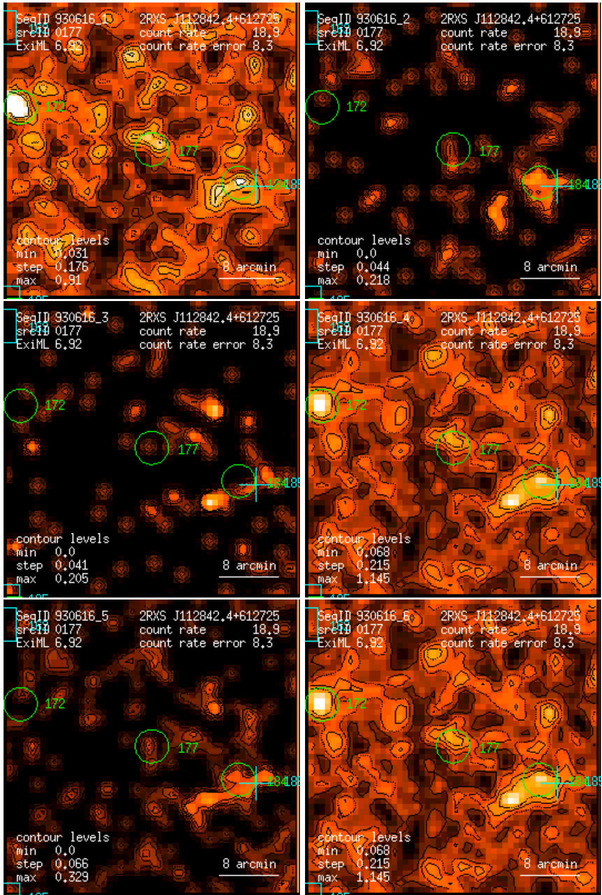
Figure 177: RASS 930616: detection 0177: band rate images, Gaussian filter: (1) PSPC channels 11 – 41, (2) 52 – 90, (3) 91 – 201, (4) 11 – 235, (5) 52 – 201, (6) 11 – 201. Broad band rates in counts/ks. Band rate contour levels in counts/ks/arcmin 2 .
