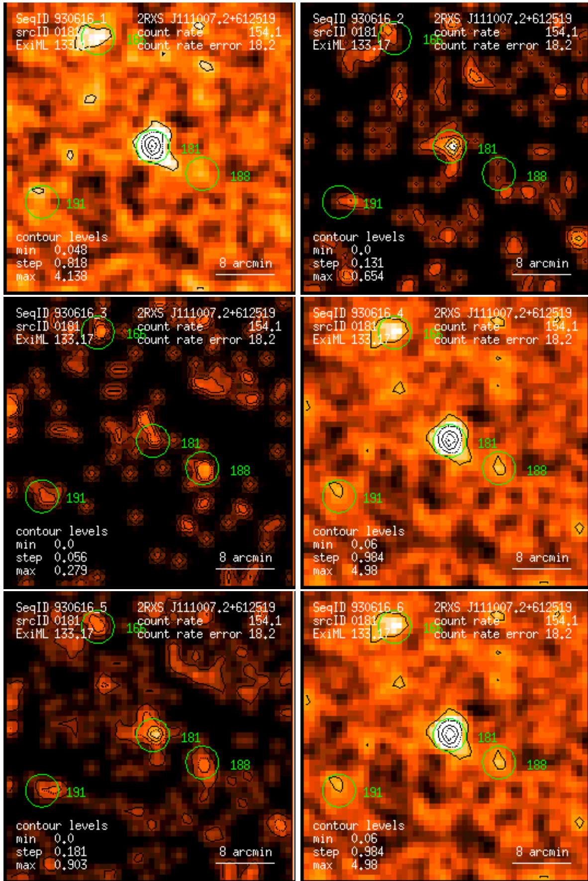
Figure 181: RASS 930616: detection 0181: band rate images, Gaussian filter: (1) PSPC channels 11 – 41, (2) 52 – 90, (3) 91 – 201, (4) 11 – 235, (5) 52 – 201, (6) 11 – 201. Broad band rates in counts/ks. Band rate contour levels in counts/ks/arcmin 2 .
