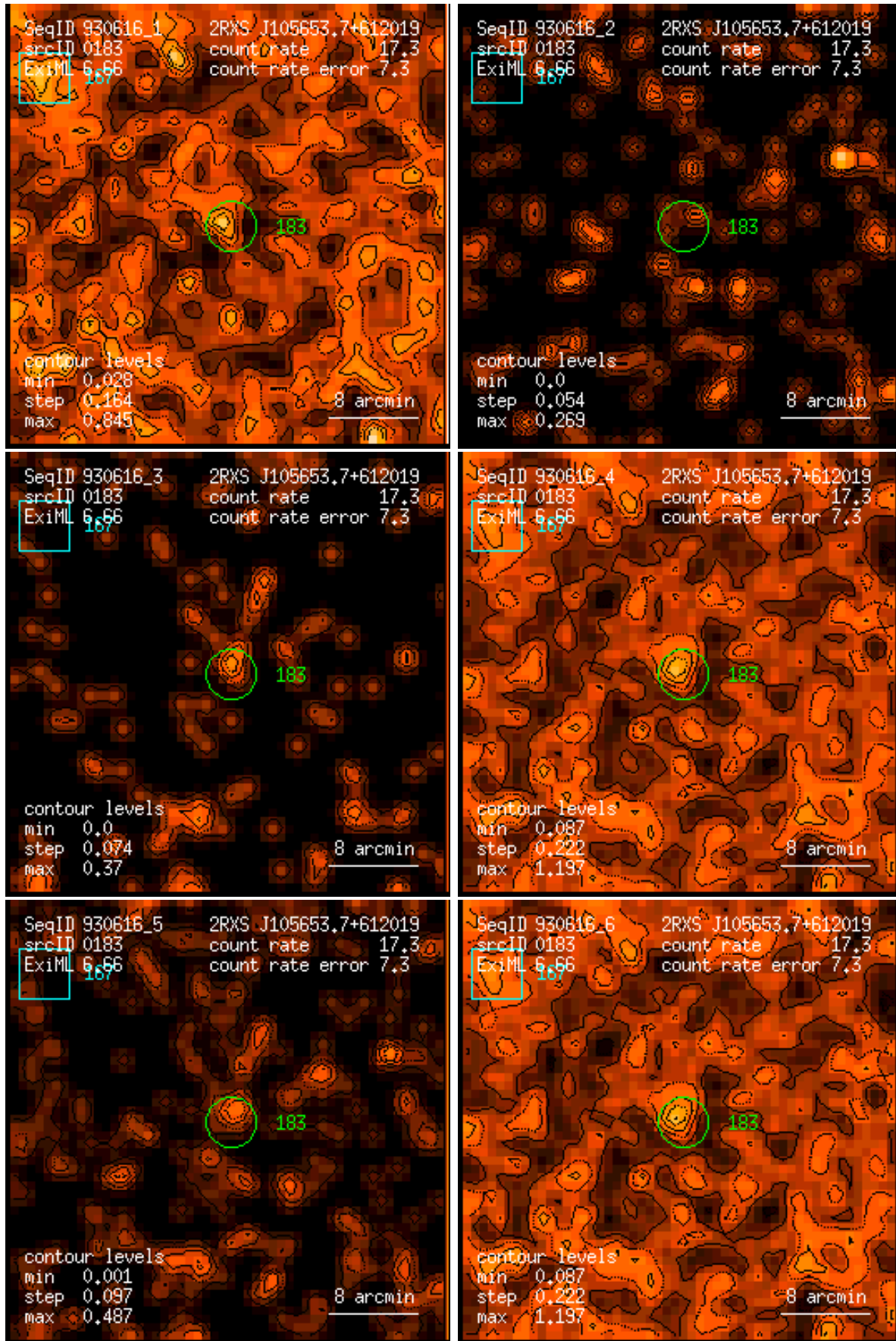
Figure 183: RASS 930616: detection 0183: band rate images, Gaussian filter: (1) PSPC channels 11 – 41, (2) 52 – 90, (3) 91 – 201, (4) 11 – 235, (5) 52 – 201, (6) 11 – 201. Broad band rates in counts/ks. Band rate contour levels in counts/ks/arcmin 2 .
