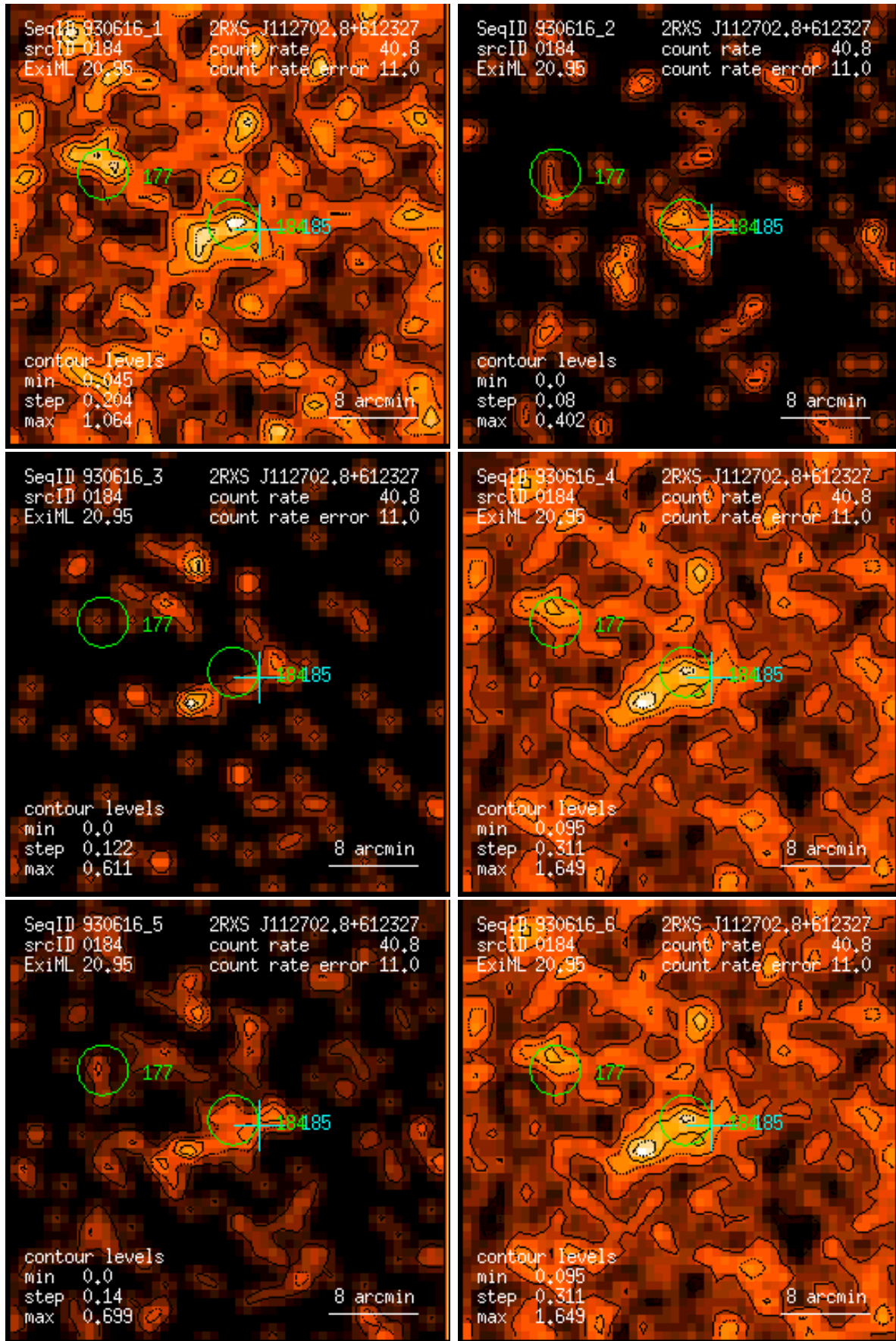
Figure 184: RASS 930616: detection 0184: band rate images, Gaussian filter: (1) PSPC channels 11 – 41, (2) 52 – 90, (3) 91 – 201, (4) 11 – 235, (5) 52 – 201, (6) 11 – 201. Broad band rates in counts/ks. Band rate contour levels in counts/ks/arcmin 2 .
