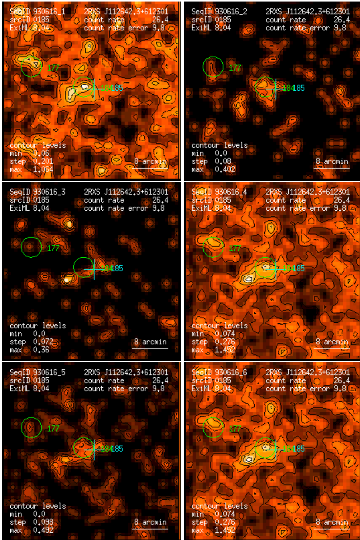
Figure 185: RASS 930616: detection 0185: band rate images, Gaussian filter: (1) PSPC channels 11 – 41, (2) 52 – 90, (3) 91 – 201, (4) 11 – 235, (5) 52 – 201, (6) 11 – 201. Broad band rates in counts/ks. Band rate contour levels in counts/ks/arcmin 2 .
