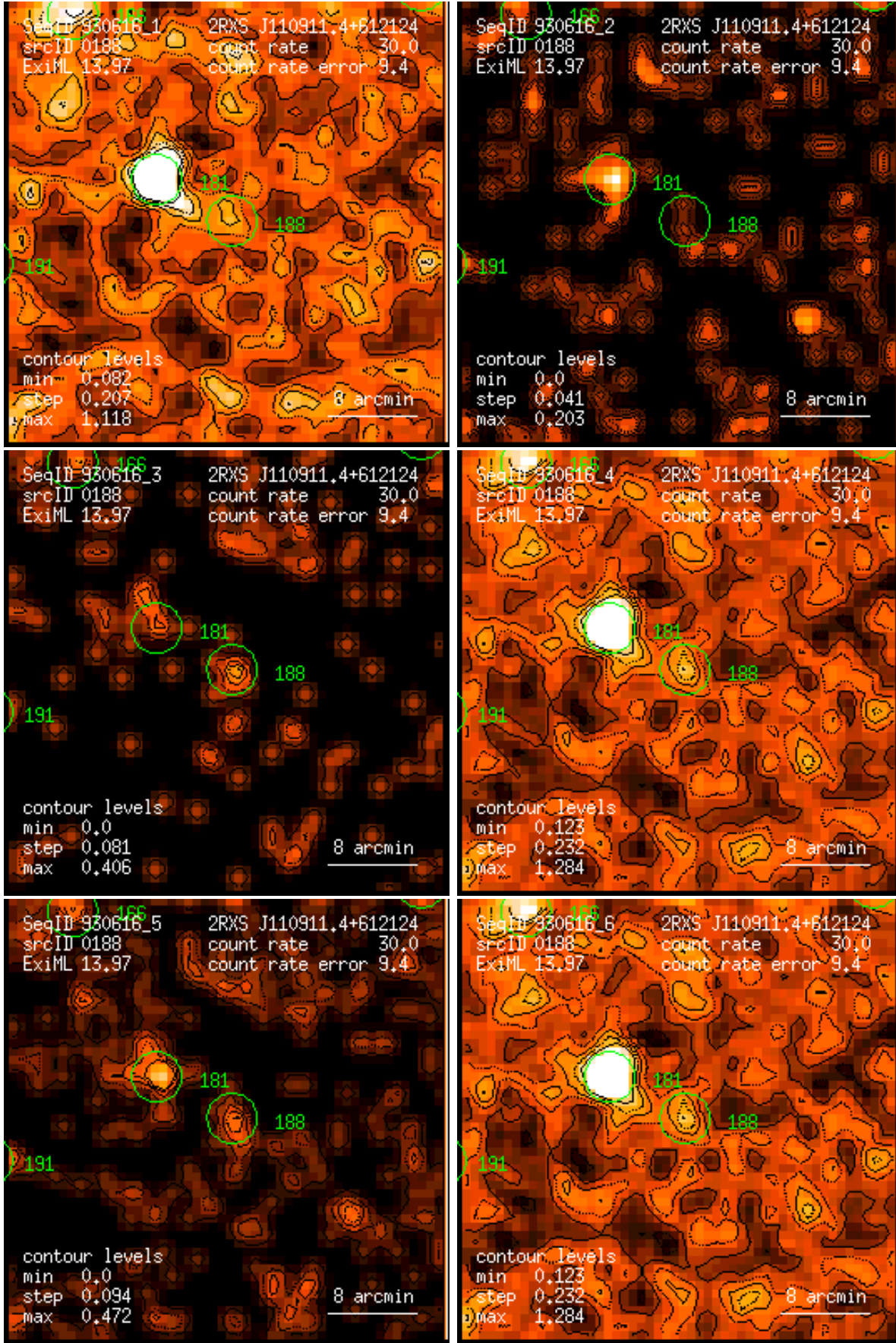
Figure 188: RASS 930616: detection 0188: band rate images, Gaussian filter: (1) PSPC channels 11 – 41, (2) 52 – 90, (3) 91 – 201, (4) 11 – 235, (5) 52 – 201, (6) 11 – 201. Broad band rates in counts/ks. Band rate contour levels in counts/ks/arcmin 2 .
