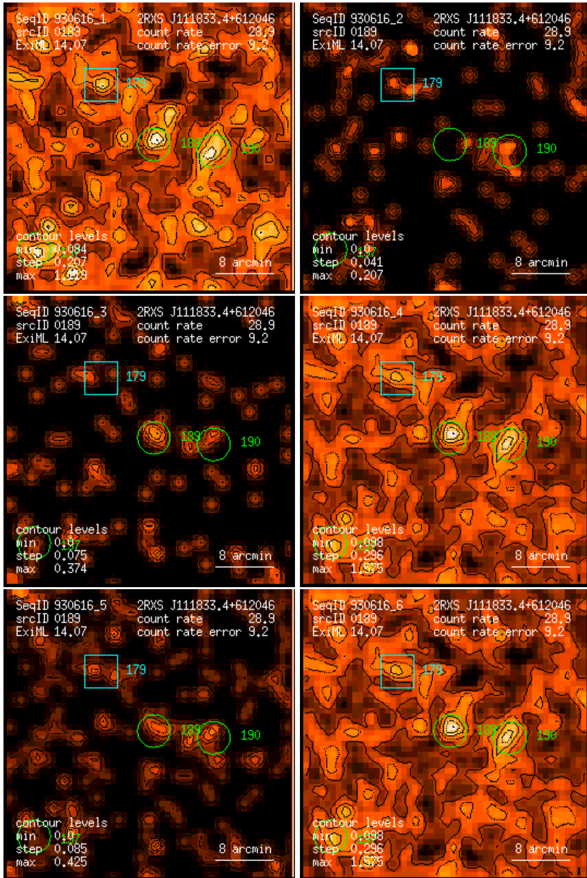
Figure 189: RASS 930616: detection 0189: band rate images, Gaussian filter: (1) PSPC channels 11 – 41, (2) 52 – 90, (3) 91 – 201, (4) 11 – 235, (5) 52 – 201, (6) 11 – 201. Broad band rates in counts/ks. Band rate contour levels in counts/ks/arcmin 2 .
