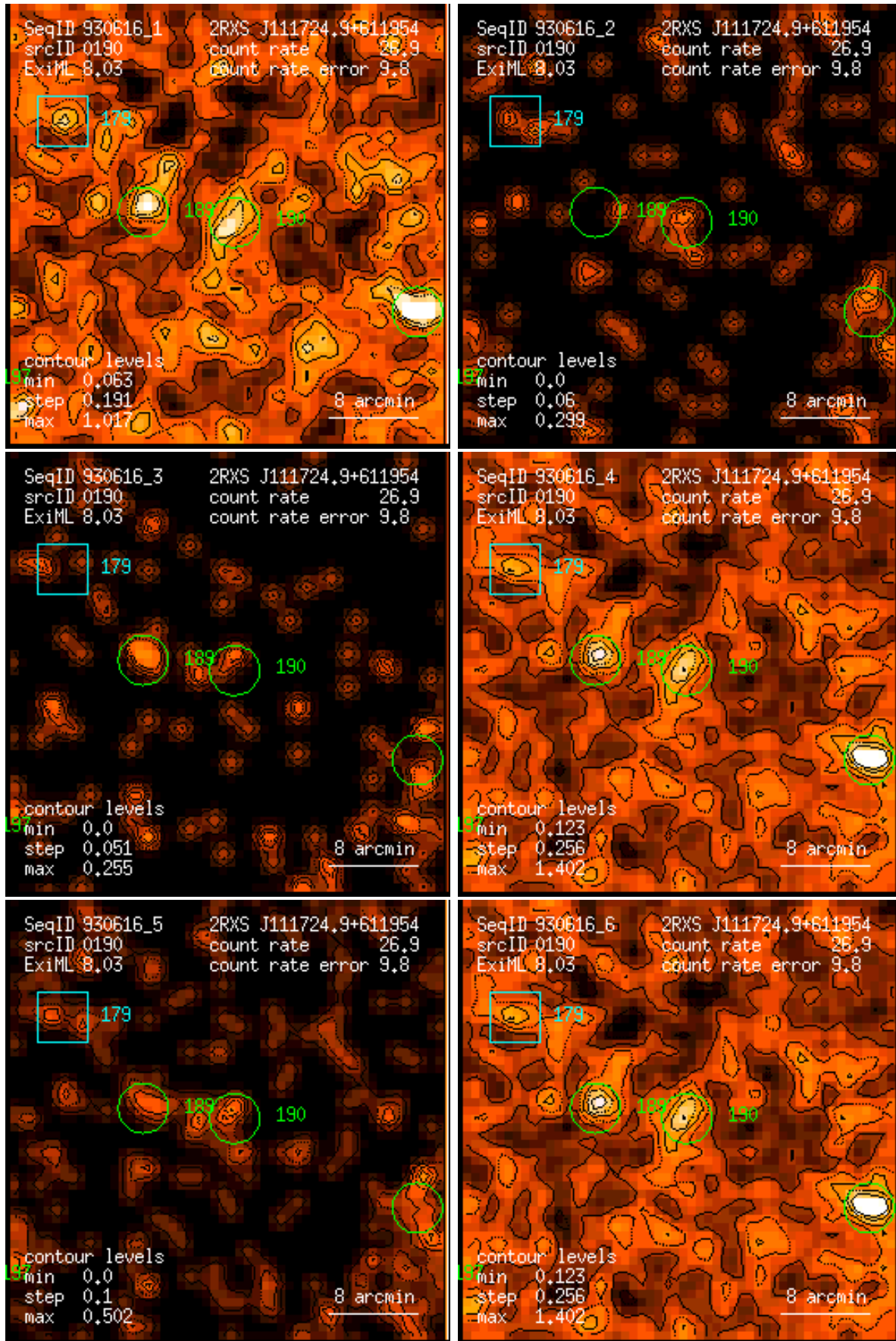
Figure 190: RASS 930616: detection 0190: band rate images, Gaussian filter: (1) PSPC channels 11 – 41, (2) 52 – 90, (3) 91 – 201, (4) 11 – 235, (5) 52 – 201, (6) 11 – 201. Broad band rates in counts/ks. Band rate contour levels in counts/ks/arcmin 2 .
