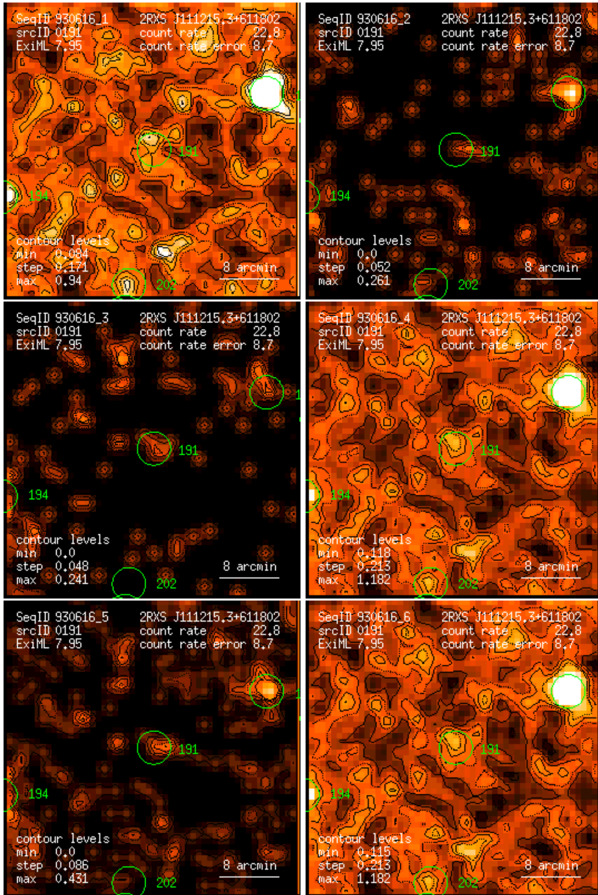
Figure 191: RASS 930616: detection 0191: band rate images, Gaussian filter: (1) PSPC channels 11 – 41, (2) 52 – 90, (3) 91 – 201, (4) 11 – 235, (5) 52 – 201, (6) 11 – 201. Broad band rates in counts/ks. Band rate contour levels in counts/ks/arcmin 2 .
