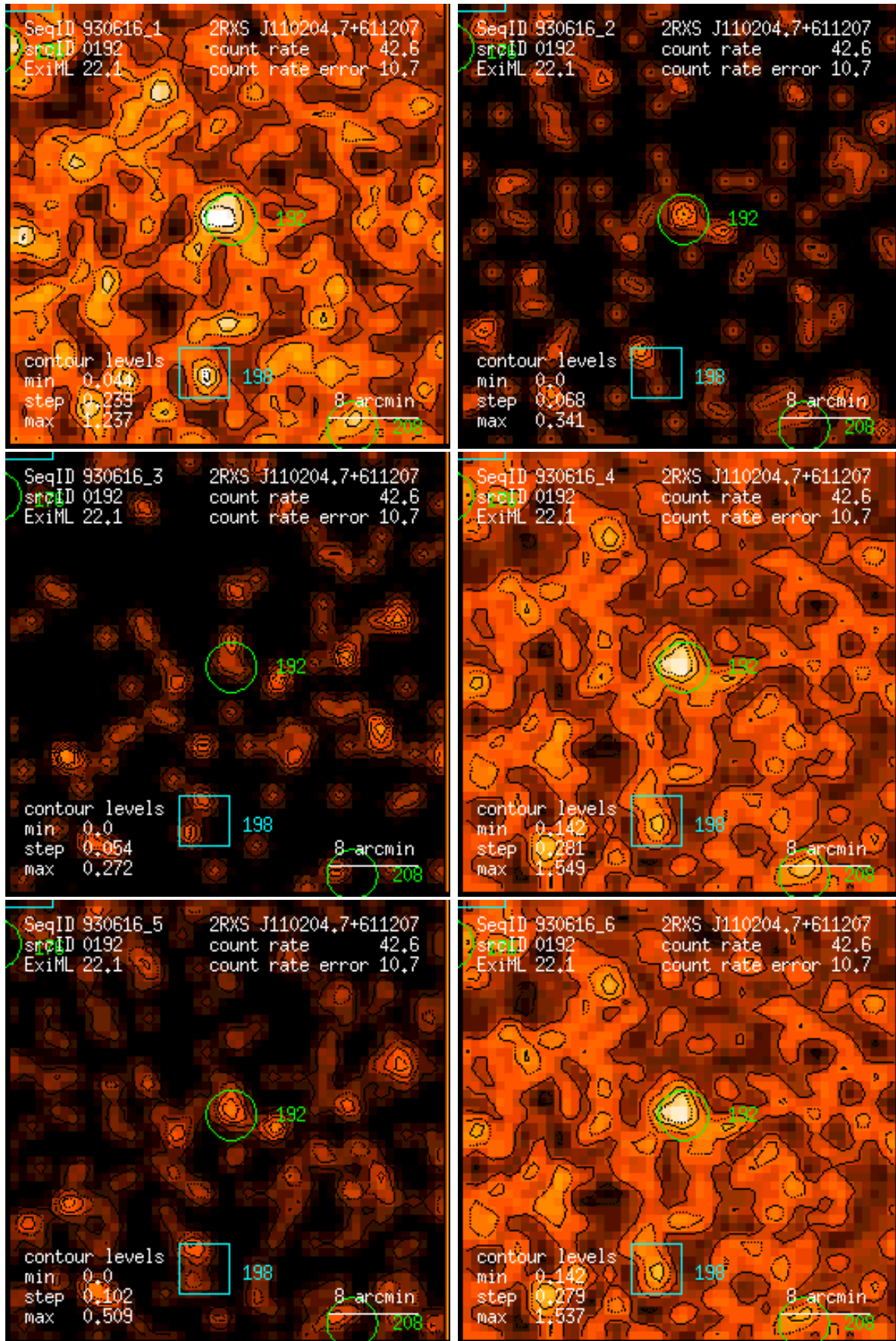
Figure 192: RASS 930616: detection 0192: band rate images, Gaussian filter: (1) PSPC channels 11 – 41, (2) 52 – 90, (3) 91 – 201, (4) 11 – 235, (5) 52 – 201, (6) 11 – 201. Broad band rates in counts/ks. Band rate contour levels in counts/ks/arcmin 2 .
