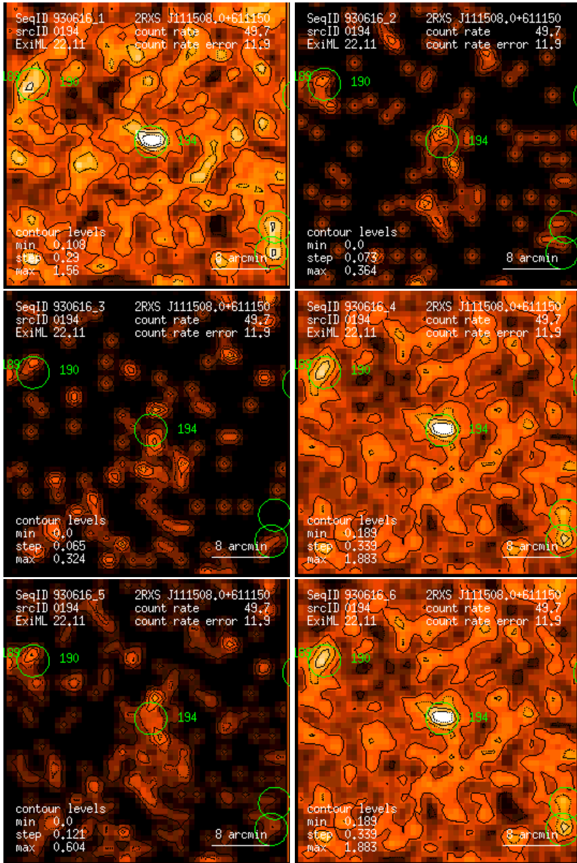
Figure 194: RASS 930616: detection 0194: band rate images, Gaussian filter: (1) PSPC channels 11 – 41, (2) 52 – 90, (3) 91 – 201, (4) 11 – 235, (5) 52 – 201, (6) 11 – 201. Broad band rates in counts/ks. Band rate contour levels in counts/ks/arcmin 2 .
