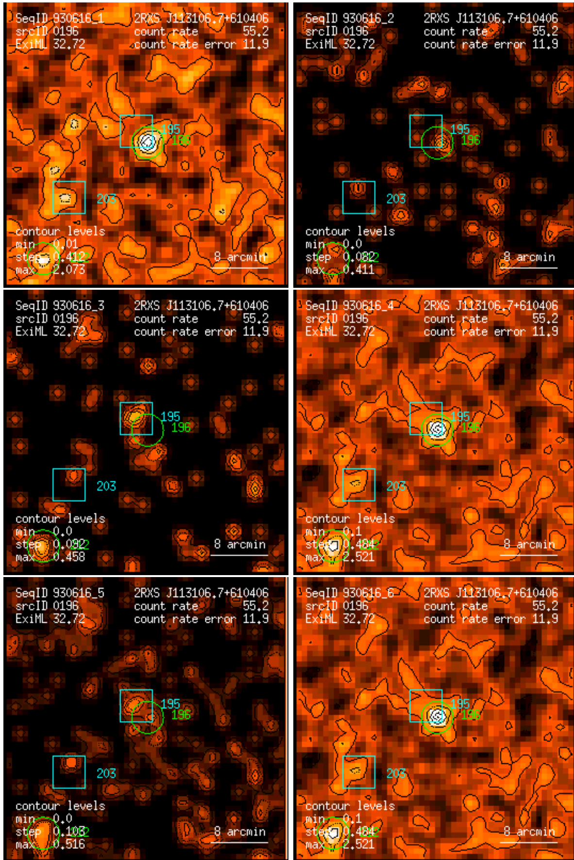
Figure 196: RASS 930616: detection 0196: band rate images, Gaussian filter: (1) PSPC channels 11 – 41, (2) 52 – 90, (3) 91 – 201, (4) 11 – 235, (5) 52 – 201, (6) 11 – 201. Broad band rates in counts/ks. Band rate contour levels in counts/ks/arcmin 2 .
