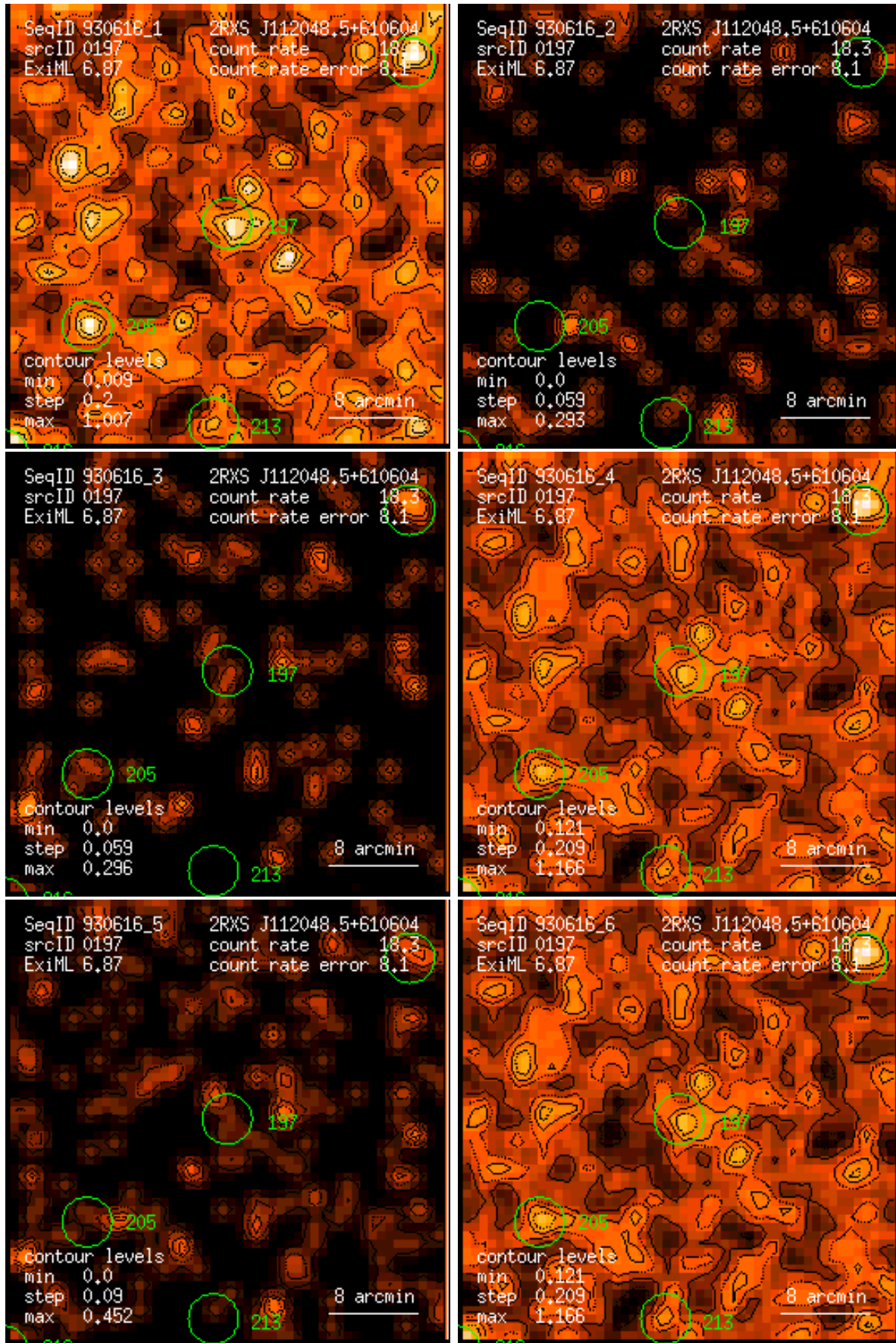
Figure 197: RASS 930616: detection 0197: band rate images, Gaussian filter: (1) PSPC channels 11 – 41, (2) 52 – 90, (3) 91 – 201, (4) 11 – 235, (5) 52 – 201, (6) 11 – 201. Broad band rates in counts/ks. Band rate contour levels in counts/ks/arcmin 2 .
