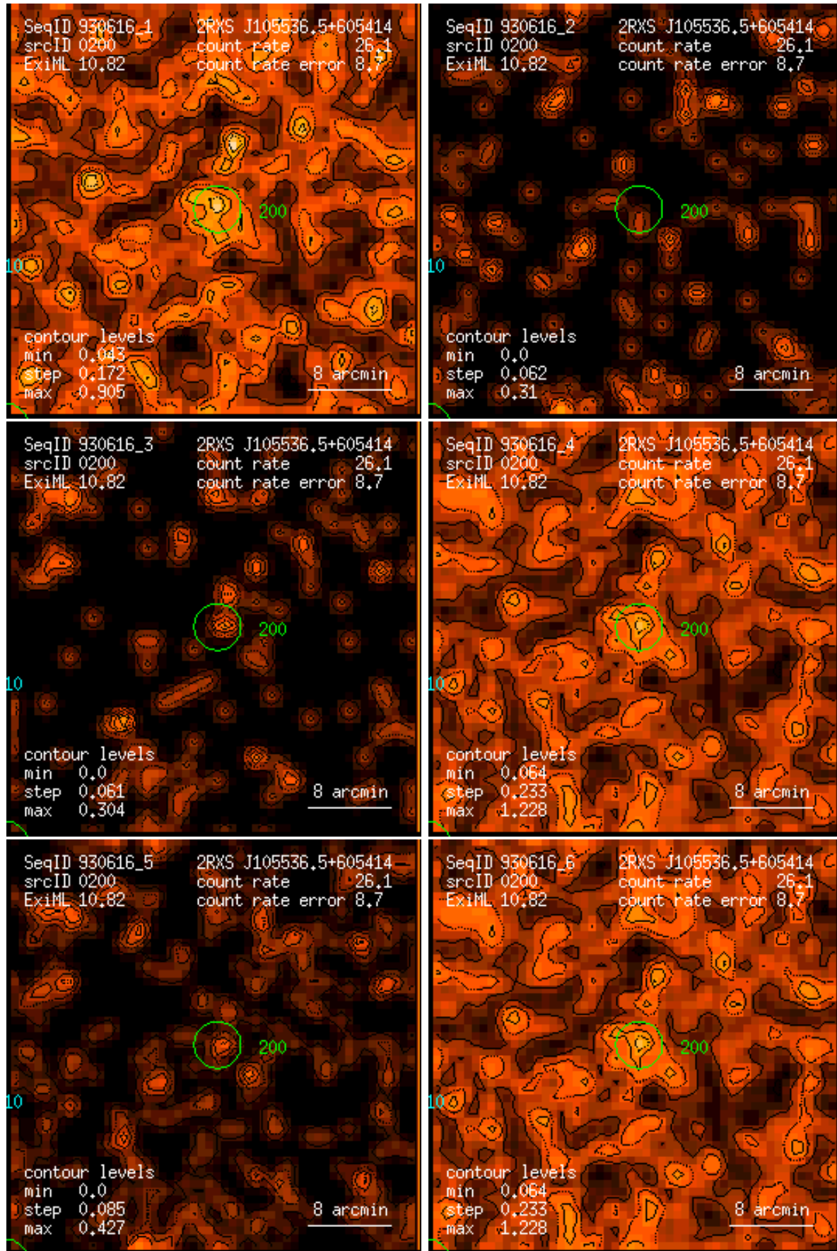
Figure 200: RASS 930616: detection 0200: band rate images, Gaussian filter: (1) PSPC channels 11 – 41, (2) 52 – 90, (3) 91 – 201, (4) 11 – 235, (5) 52 – 201, (6) 11 – 201. Broad band rates in counts/ks. Band rate contour levels in counts/ks/arcmin 2 .
