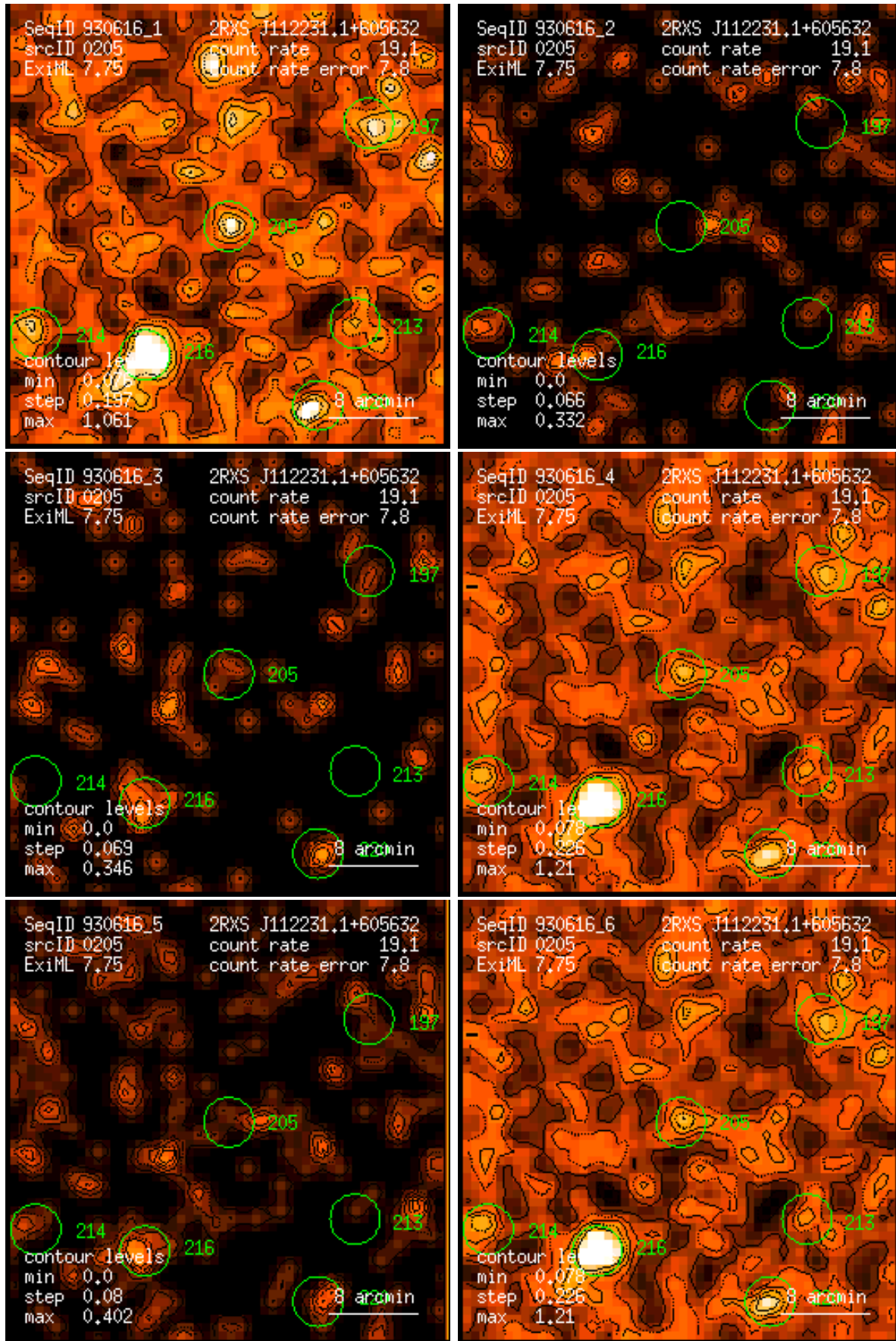
Figure 205: RASS 930616: detection 0205: band rate images, Gaussian filter: (1) PSPC channels 11 – 41, (2) 52 – 90, (3) 91 – 201, (4) 11 – 235, (5) 52 – 201, (6) 11 – 201. Broad band rates in counts/ks. Band rate contour levels in counts/ks/arcmin 2 .
