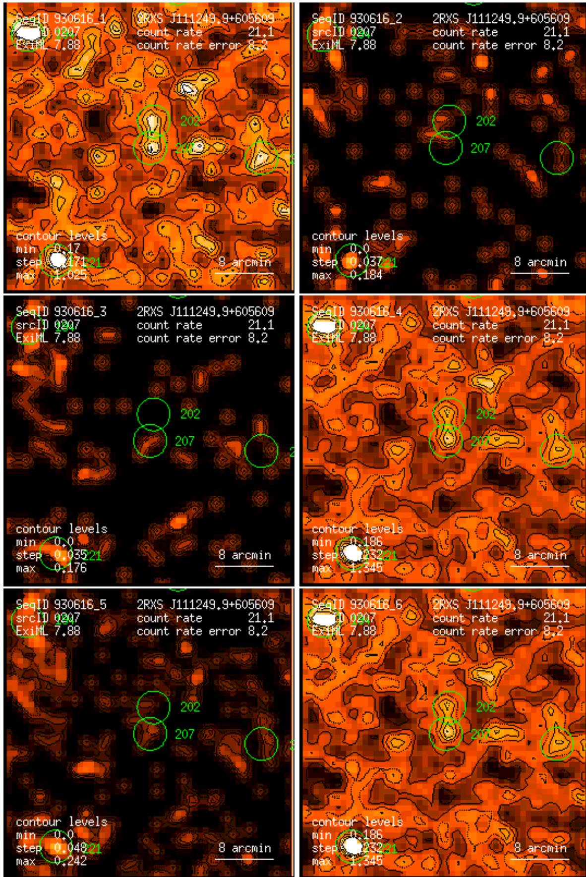
Figure 207: RASS 930616: detection 0207: band rate images, Gaussian filter: (1) PSPC channels 11 – 41, (2) 52 – 90, (3) 91 – 201, (4) 11 – 235, (5) 52 – 201, (6) 11 – 201. Broad band rates in counts/ks. Band rate contour levels in counts/ks/arcmin 2 .
