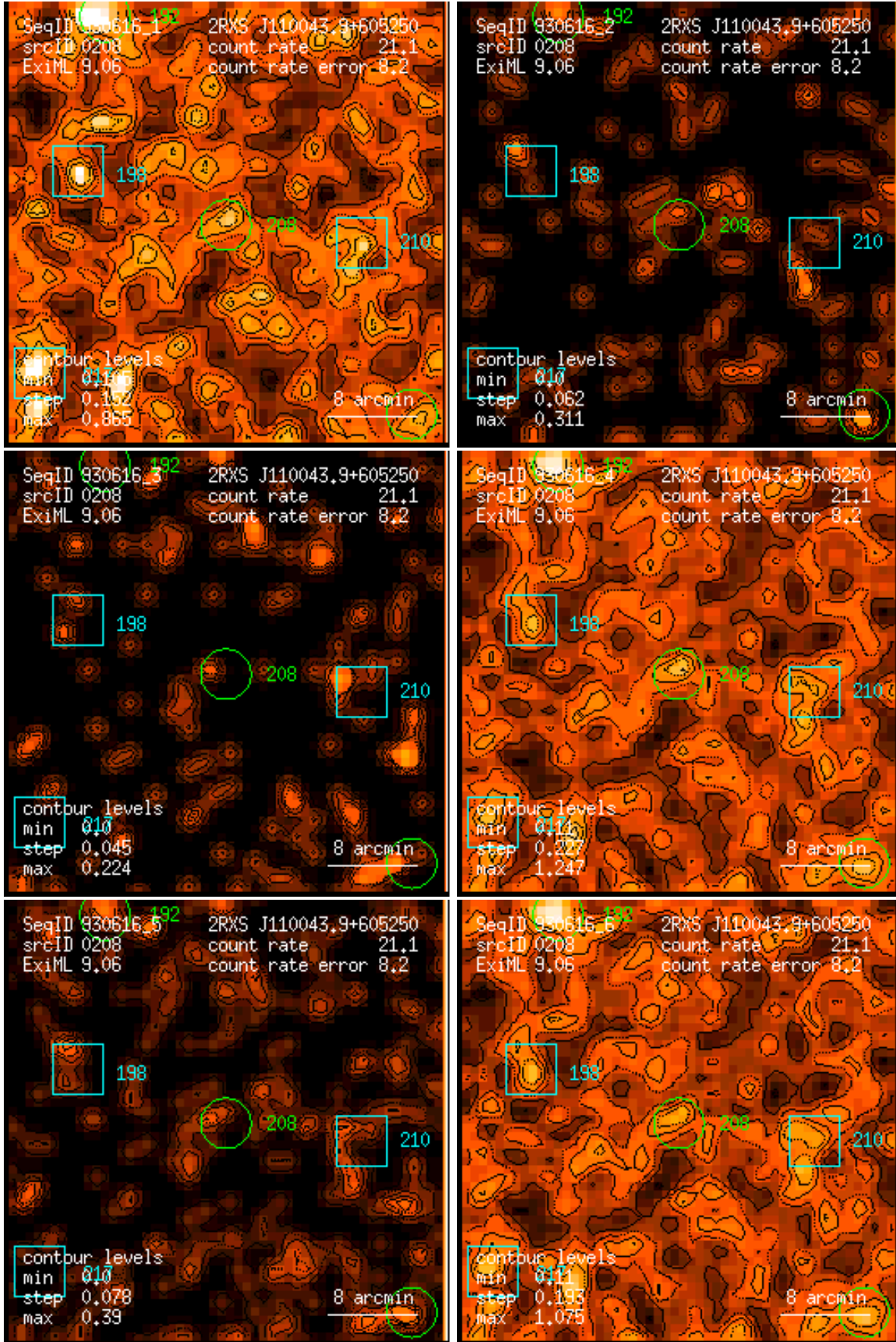
Figure 208: RASS 930616: detection 0208: band rate images, Gaussian filter: (1) PSPC channels 11 – 41, (2) 52 – 90, (3) 91 – 201, (4) 11 – 235, (5) 52 – 201, (6) 11 – 201. Broad band rates in counts/ks. Band rate contour levels in counts/ks/arcmin 2 .
