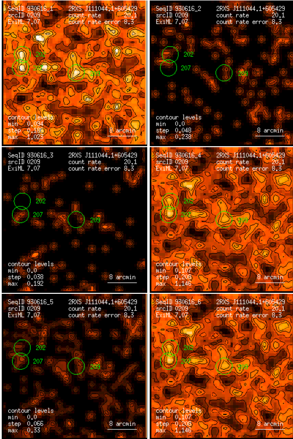
Figure 209: RASS 930616: detection 0209: band rate images, Gaussian filter: (1) PSPC channels 11 – 41, (2) 52 – 90, (3) 91 – 201, (4) 11 – 235, (5) 52 – 201, (6) 11 – 201. Broad band rates in counts/ks. Band rate contour levels in counts/ks/arcmin 2 .
