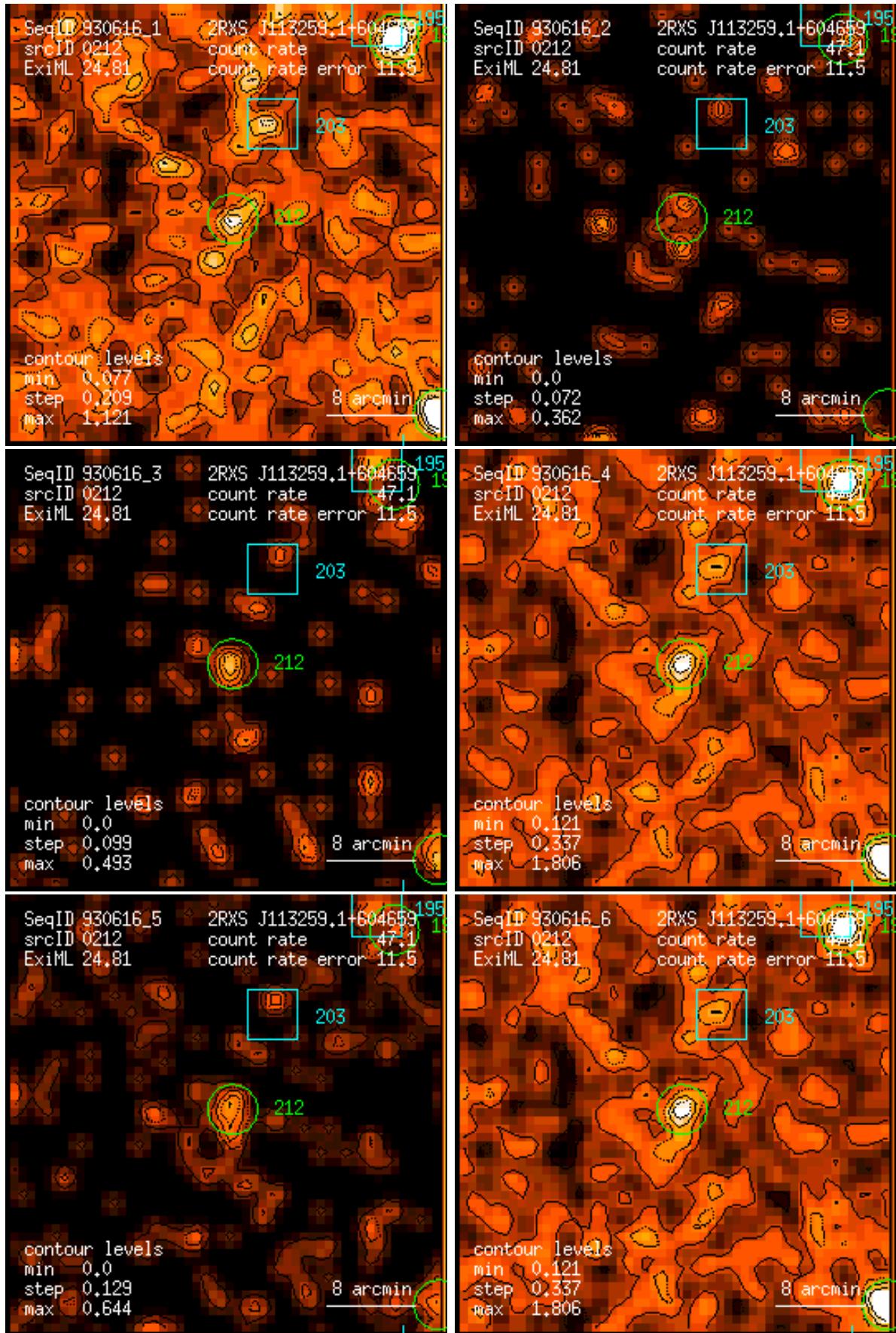
Figure 212: RASS 930616: detection 0212: band rate images, Gaussian filter: (1) PSPC channels 11 – 41, (2) 52 – 90, (3) 91 – 201, (4) 11 – 235, (5) 52 – 201, (6) 11 – 201. Broad band rates in counts/ks. Band rate contour levels in counts/ks/arcmin 2 .
