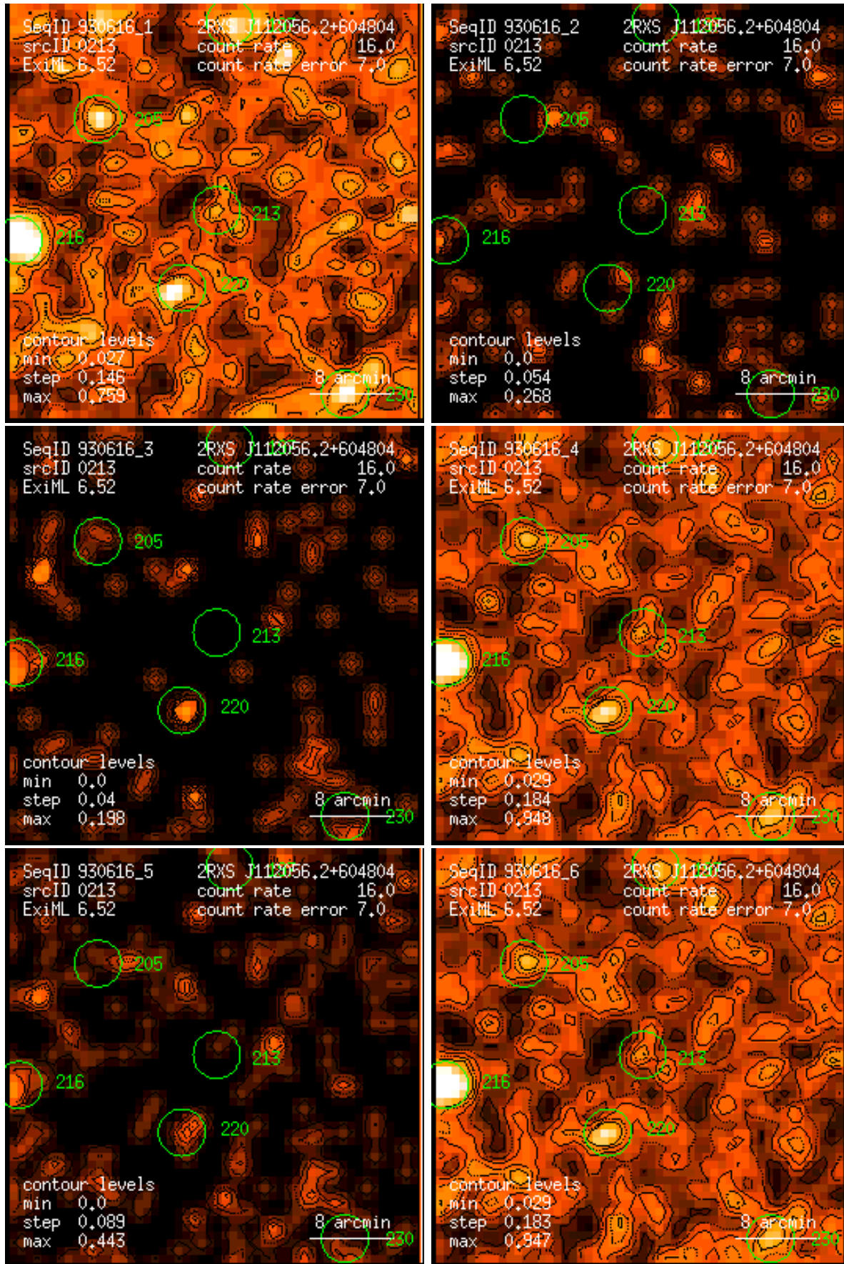
Figure 213: RASS 930616: detection 0213: band rate images, Gaussian filter: (1) PSPC channels 11 – 41, (2) 52 – 90, (3) 91 – 201, (4) 11 – 235, (5) 52 – 201, (6) 11 – 201. Broad band rates in counts/ks. Band rate contour levels in counts/ks/arcmin 2 .
