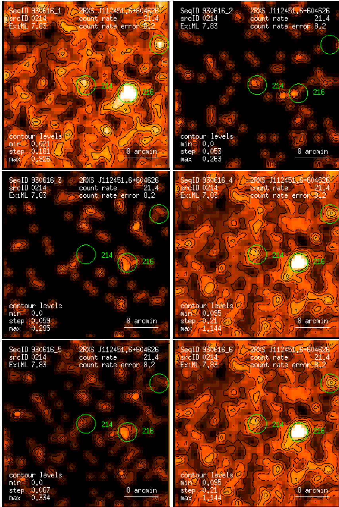
Figure 214: RASS 930616: detection 0214: band rate images, Gaussian filter: (1) PSPC channels 11 – 41, (2) 52 – 90, (3) 91 – 201, (4) 11 – 235, (5) 52 – 201, (6) 11 – 201. Broad band rates in counts/ks. Band rate contour levels in counts/ks/arcmin 2 .
