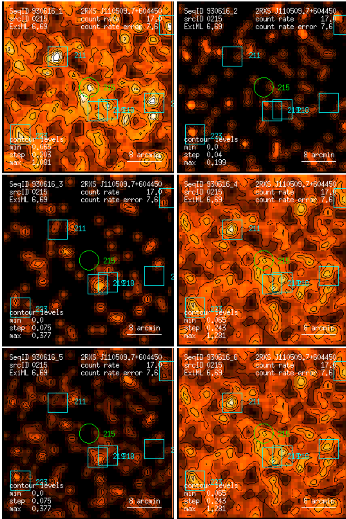
Figure 215: RASS 930616: detection 0215: band rate images, Gaussian filter: (1) PSPC channels 11 – 41, (2) 52 – 90, (3) 91 – 201, (4) 11 – 235, (5) 52 – 201, (6) 11 – 201. Broad band rates in counts/ks. Band rate contour levels in counts/ks/arcmin 2 .
