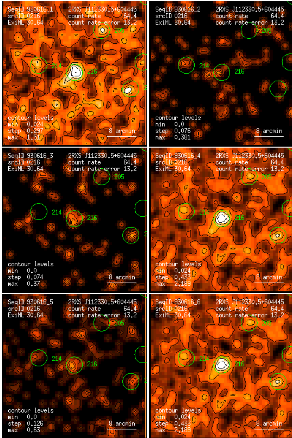
Figure 216: RASS 930616: detection 0216: band rate images, Gaussian filter: (1) PSPC channels 11 – 41, (2) 52 – 90, (3) 91 – 201, (4) 11 – 235, (5) 52 – 201, (6) 11 – 201. Broad band rates in counts/ks. Band rate contour levels in counts/ks/arcmin 2 .
