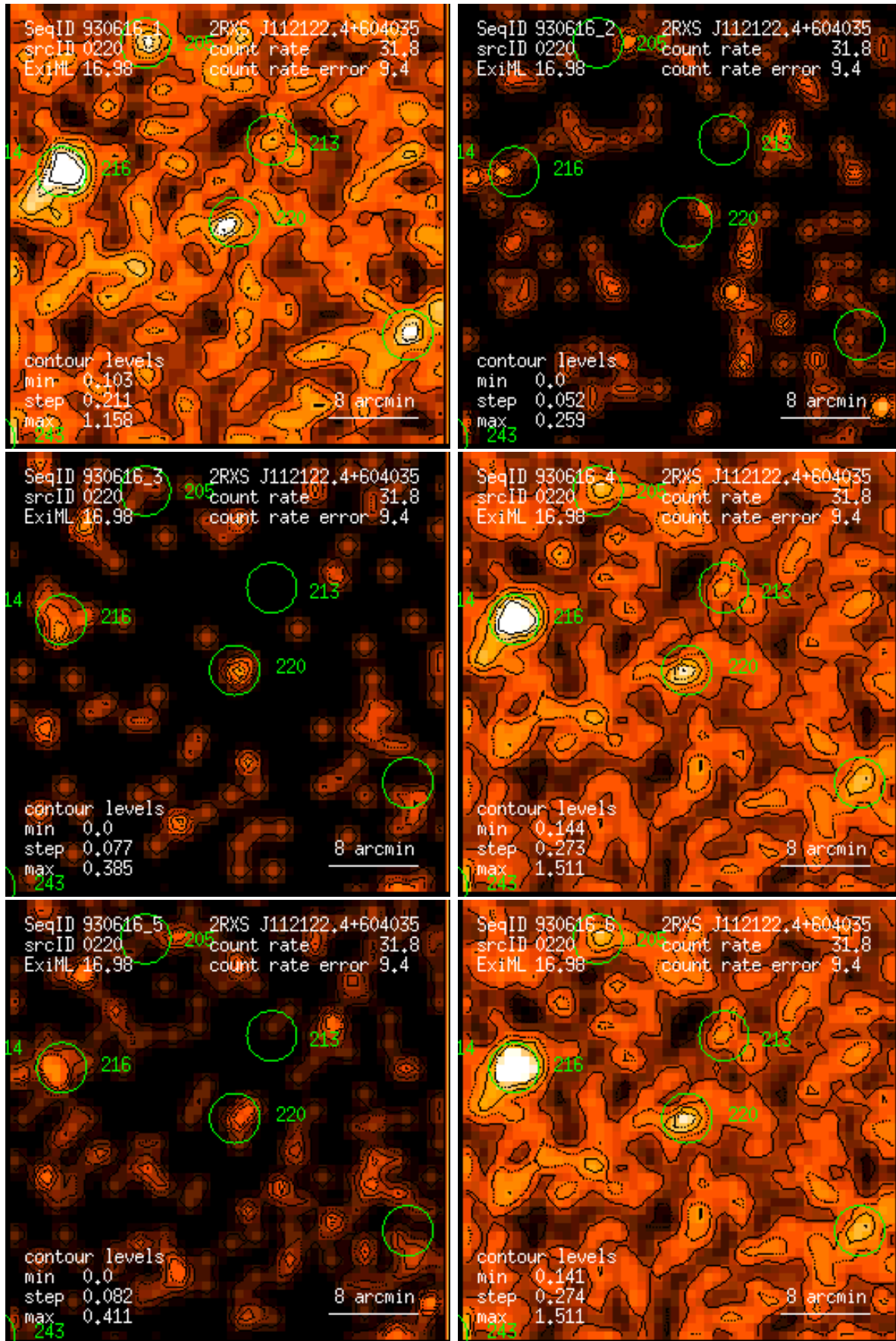
Figure 220: RASS 930616: detection 0220: band rate images, Gaussian filter: (1) PSPC channels 11 – 41, (2) 52 – 90, (3) 91 – 201, (4) 11 – 235, (5) 52 – 201, (6) 11 – 201. Broad band rates in counts/ks. Band rate contour levels in counts/ks/arcmin 2 .
