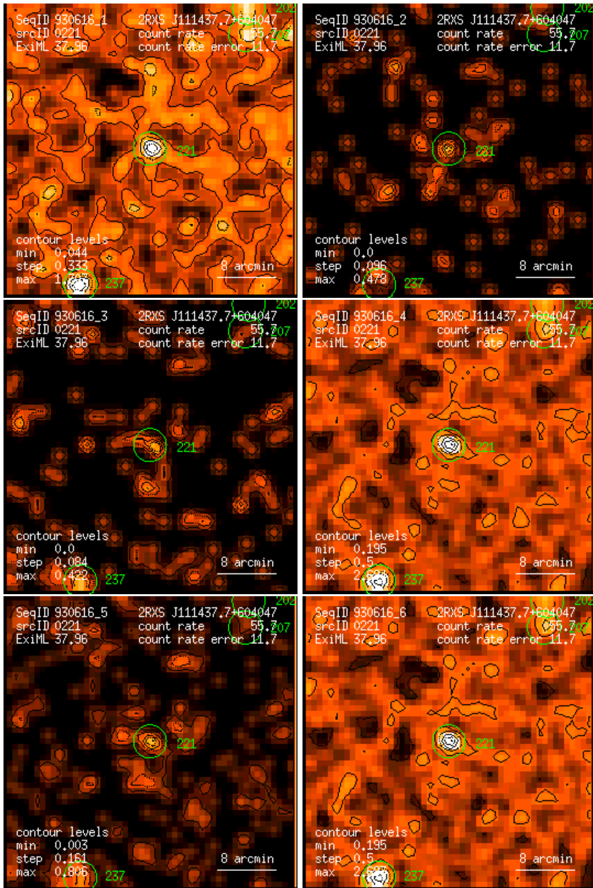
Figure 221: RASS 930616: detection 0221: band rate images, Gaussian filter: (1) PSPC channels 11 – 41, (2) 52 – 90, (3) 91 – 201, (4) 11 – 235, (5) 52 – 201, (6) 11 – 201. Broad band rates in counts/ks. Band rate contour levels in counts/ks/arcmin 2 .
