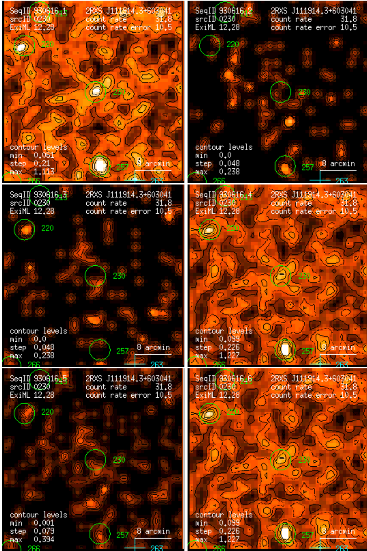
Figure 230: RASS 930616: detection 0230: band rate images, Gaussian filter: (1) PSPC channels 11 – 41, (2) 52 – 90, (3) 91 – 201, (4) 11 – 235, (5) 52 – 201, (6) 11 – 201. Broad band rates in counts/ks. Band rate contour levels in counts/ks/arcmin 2 .
