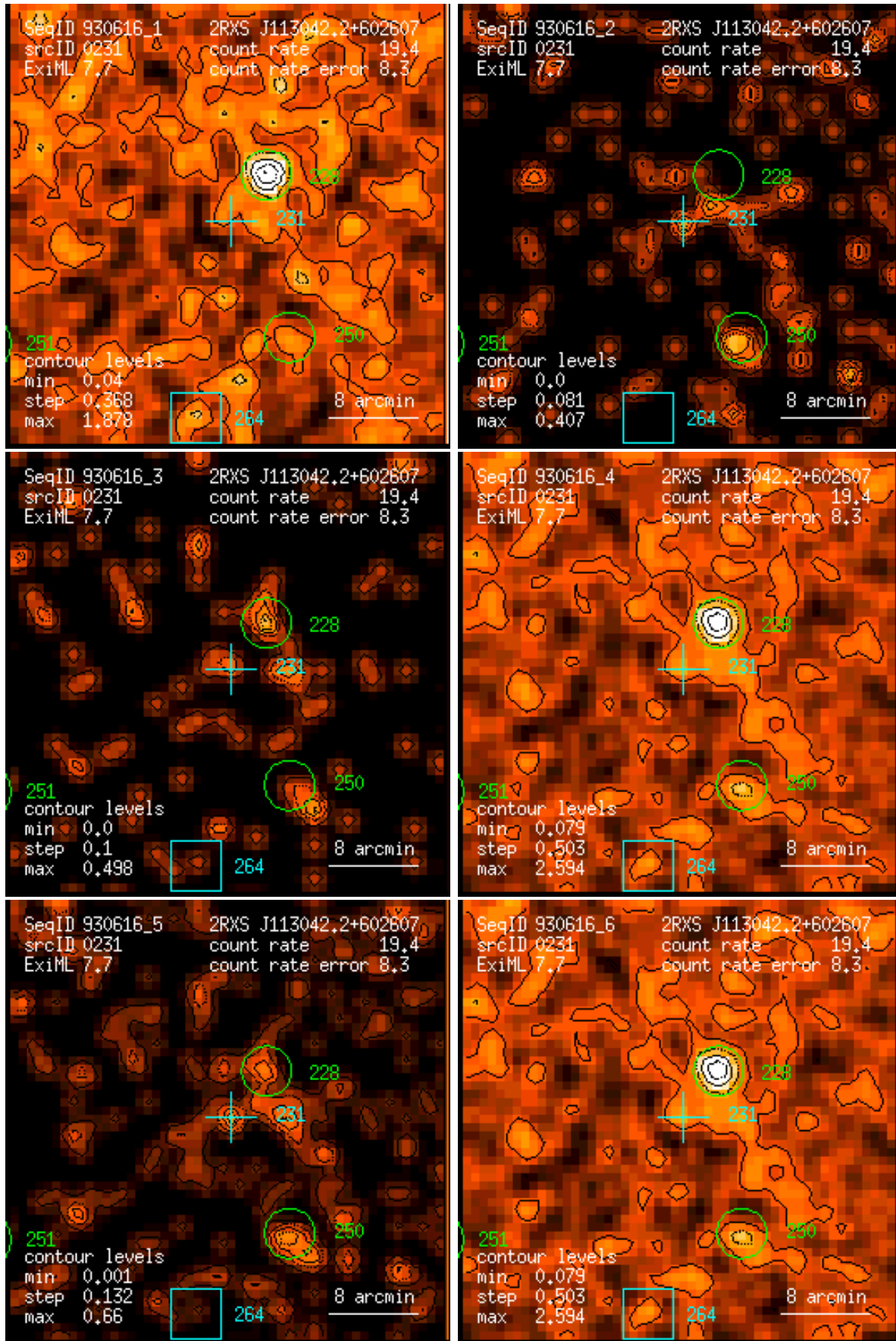
Figure 231: RASS 930616: detection 0231: band rate images, Gaussian filter: (1) PSPC channels 11 – 41, (2) 52 – 90, (3) 91 – 201, (4) 11 – 235, (5) 52 – 201, (6) 11 – 201. Broad band rates in counts/ks. Band rate contour levels in counts/ks/arcmin 2 .
