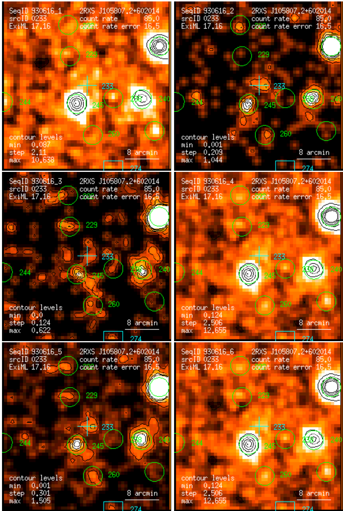
Figure 233: RASS 930616: detection 0233: band rate images, Gaussian filter: (1) PSPC channels 11 – 41, (2) 52 – 90, (3) 91 – 201, (4) 11 – 235, (5) 52 – 201, (6) 11 – 201. Broad band rates in counts/ks. Band rate contour levels in counts/ks/arcmin 2 .
