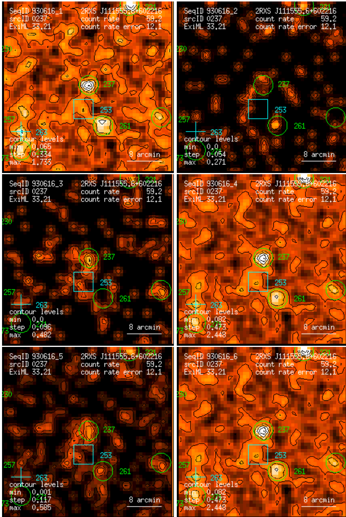
Figure 237: RASS 930616: detection 0237: band rate images, Gaussian filter: (1) PSPC channels 11 – 41, (2) 52 – 90, (3) 91 – 201, (4) 11 – 235, (5) 52 – 201, (6) 11 – 201. Broad band rates in counts/ks. Band rate contour levels in counts/ks/arcmin 2 .
