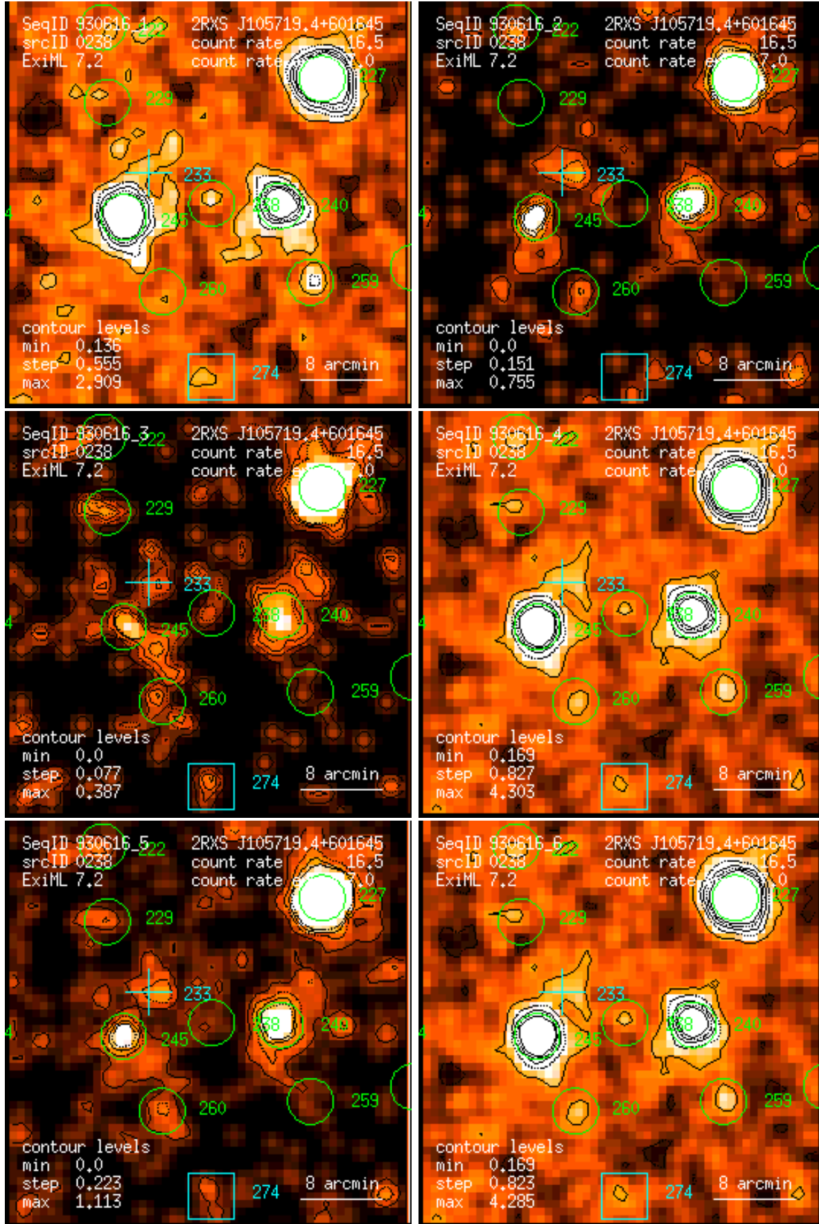
Figure 238: RASS 930616: detection 0238: band rate images, Gaussian filter: (1) PSPC channels 11 – 41, (2) 52 – 90, (3) 91 – 201, (4) 11 – 235, (5) 52 – 201, (6) 11 – 201. Broad band rates in counts/ks. Band rate contour levels in counts/ks/arcmin 2 .
