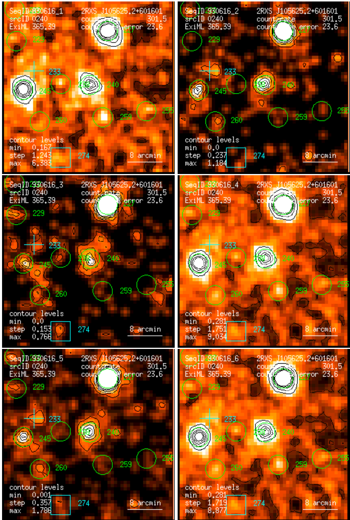
Figure 240: RASS 930616: detection 0240: band rate images, Gaussian filter: (1) PSPC channels 11 – 41, (2) 52 – 90, (3) 91 – 201, (4) 11 – 235, (5) 52 – 201, (6) 11 – 201. Broad band rates in counts/ks. Band rate contour levels in counts/ks/arcmin 2 .
