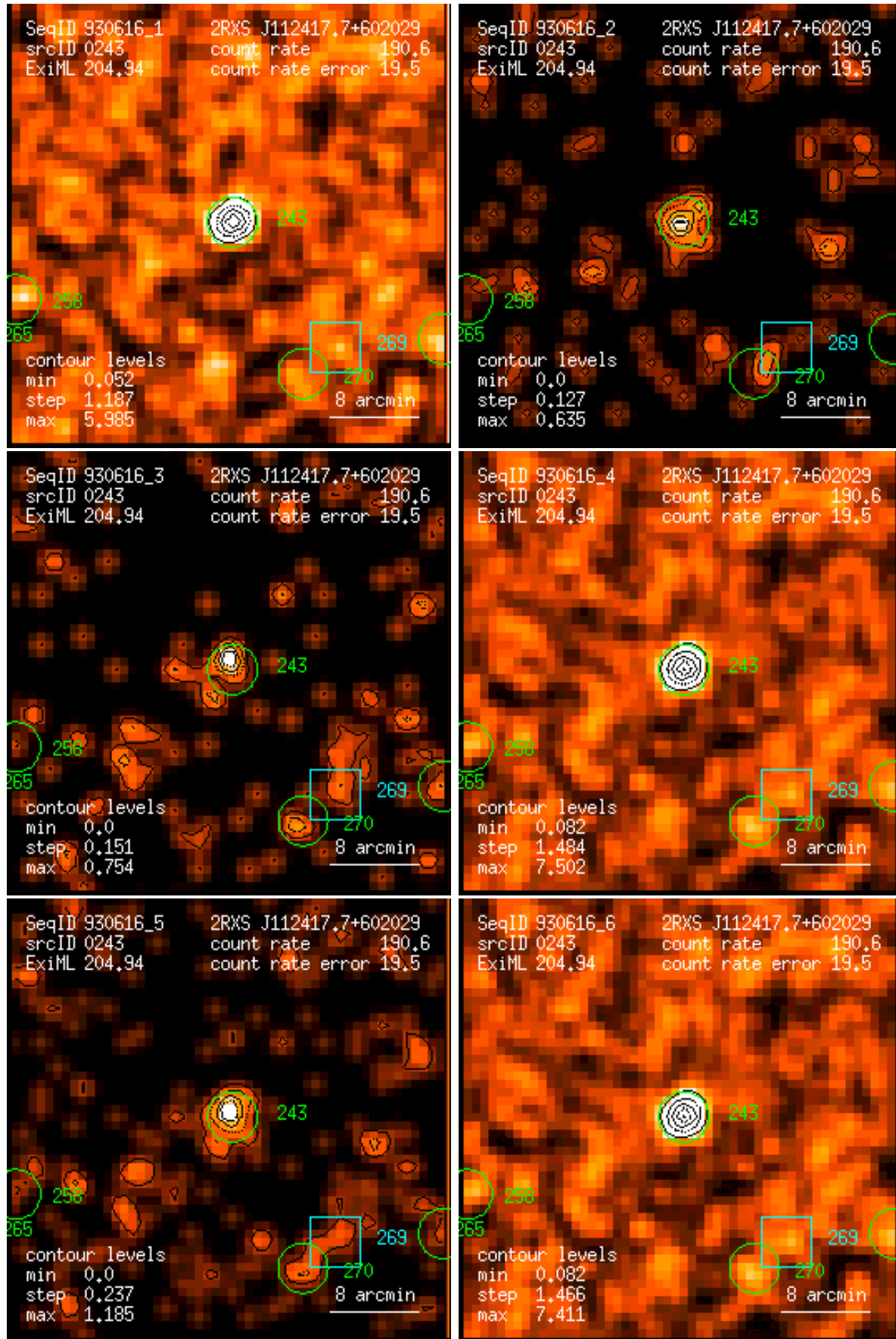
Figure 243: RASS 930616: detection 0243: band rate images, Gaussian filter: (1) PSPC channels 11 – 41, (2) 52 – 90, (3) 91 – 201, (4) 11 – 235, (5) 52 – 201, (6) 11 – 201. Broad band rates in counts/ks. Band rate contour levels in counts/ks/arcmin 2 .
