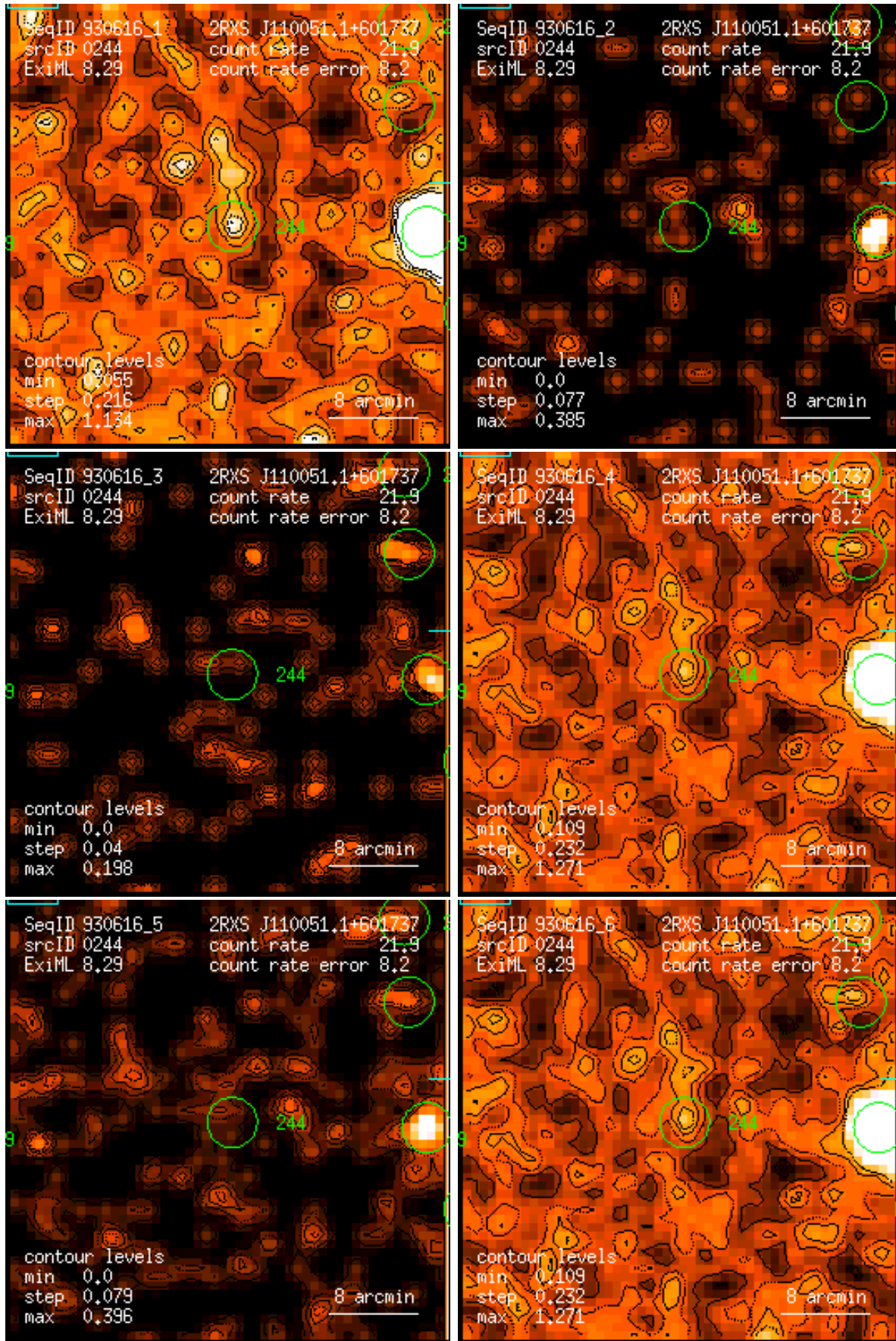
Figure 244: RASS 930616: detection 0244: band rate images, Gaussian filter: (1) PSPC channels 11 – 41, (2) 52 – 90, (3) 91 – 201, (4) 11 – 235, (5) 52 – 201, (6) 11 – 201. Broad band rates in counts/ks. Band rate contour levels in counts/ks/arcmin 2 .
