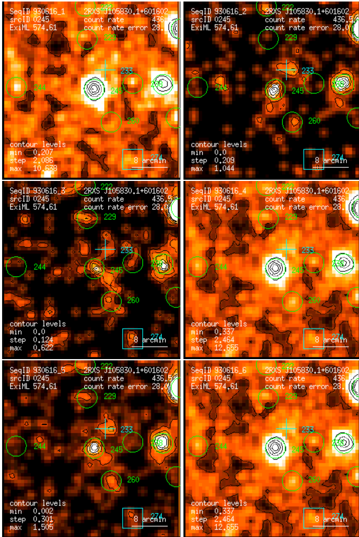
Figure 245: RASS 930616: detection 0245: band rate images, Gaussian filter: (1) PSPC channels 11 – 41, (2) 52 – 90, (3) 91 – 201, (4) 11 – 235, (5) 52 – 201, (6) 11 – 201. Broad band rates in counts/ks. Band rate contour levels in counts/ks/arcmin 2 .
