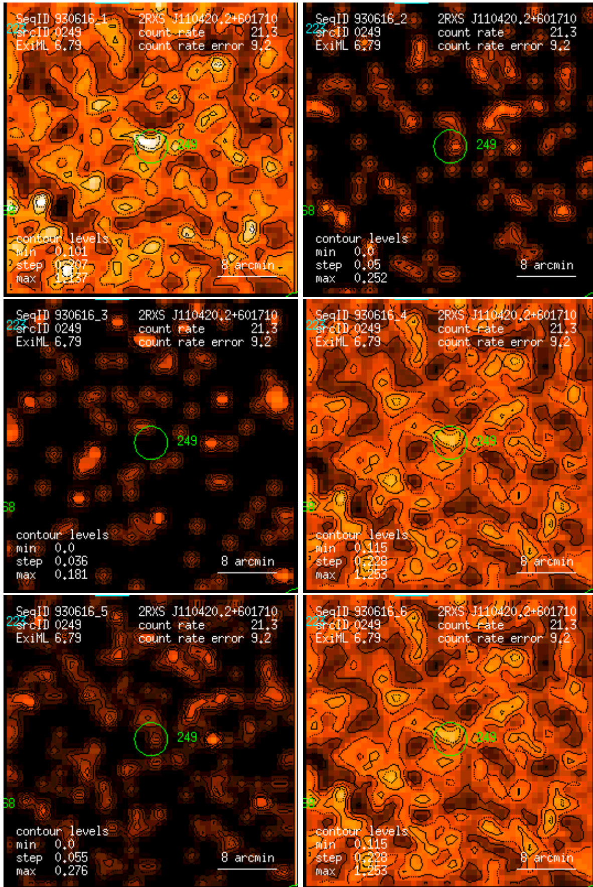
Figure 249: RASS 930616: detection 0249: band rate images, Gaussian filter: (1) PSPC channels 11 – 41, (2) 52 – 90, (3) 91 – 201, (4) 11 – 235, (5) 52 – 201, (6) 11 – 201. Broad band rates in counts/ks. Band rate contour levels in counts/ks/arcmin 2 .
