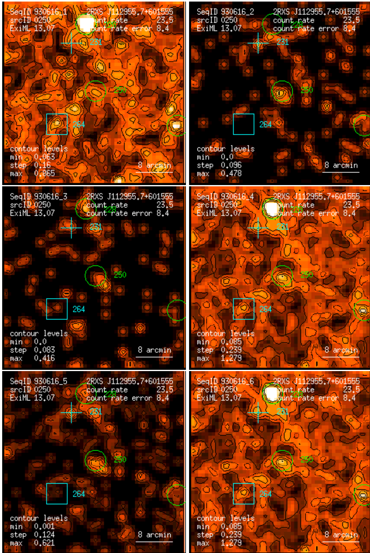
Figure 250: RASS 930616: detection 0250: band rate images, Gaussian filter: (1) PSPC channels 11 – 41, (2) 52 – 90, (3) 91 – 201, (4) 11 – 235, (5) 52 – 201, (6) 11 – 201. Broad band rates in counts/ks. Band rate contour levels in counts/ks/arcmin 2 .
