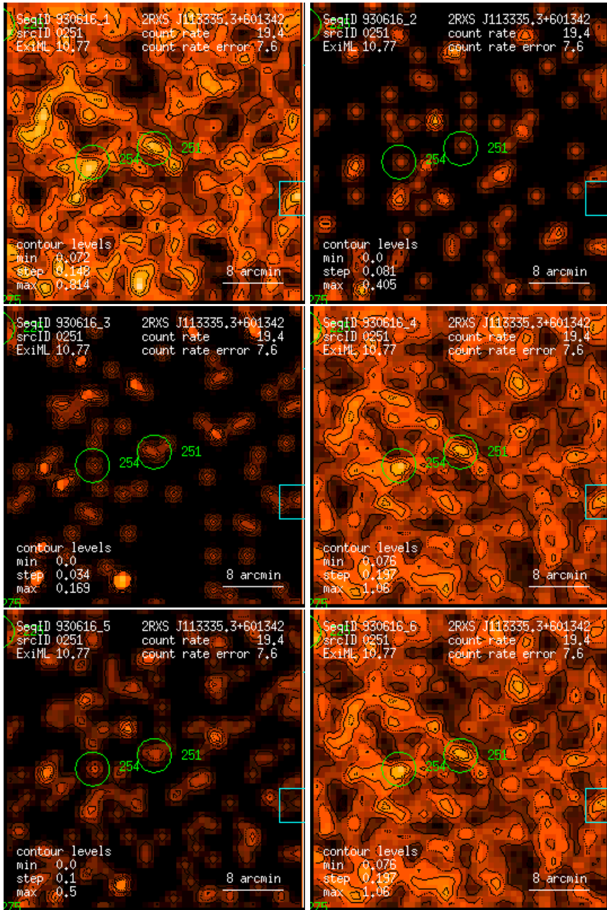
Figure 251: RASS 930616: detection 0251: band rate images, Gaussian filter: (1) PSPC channels 11 – 41, (2) 52 – 90, (3) 91 – 201, (4) 11 – 235, (5) 52 – 201, (6) 11 – 201. Broad band rates in counts/ks. Band rate contour levels in counts/ks/arcmin 2 .
