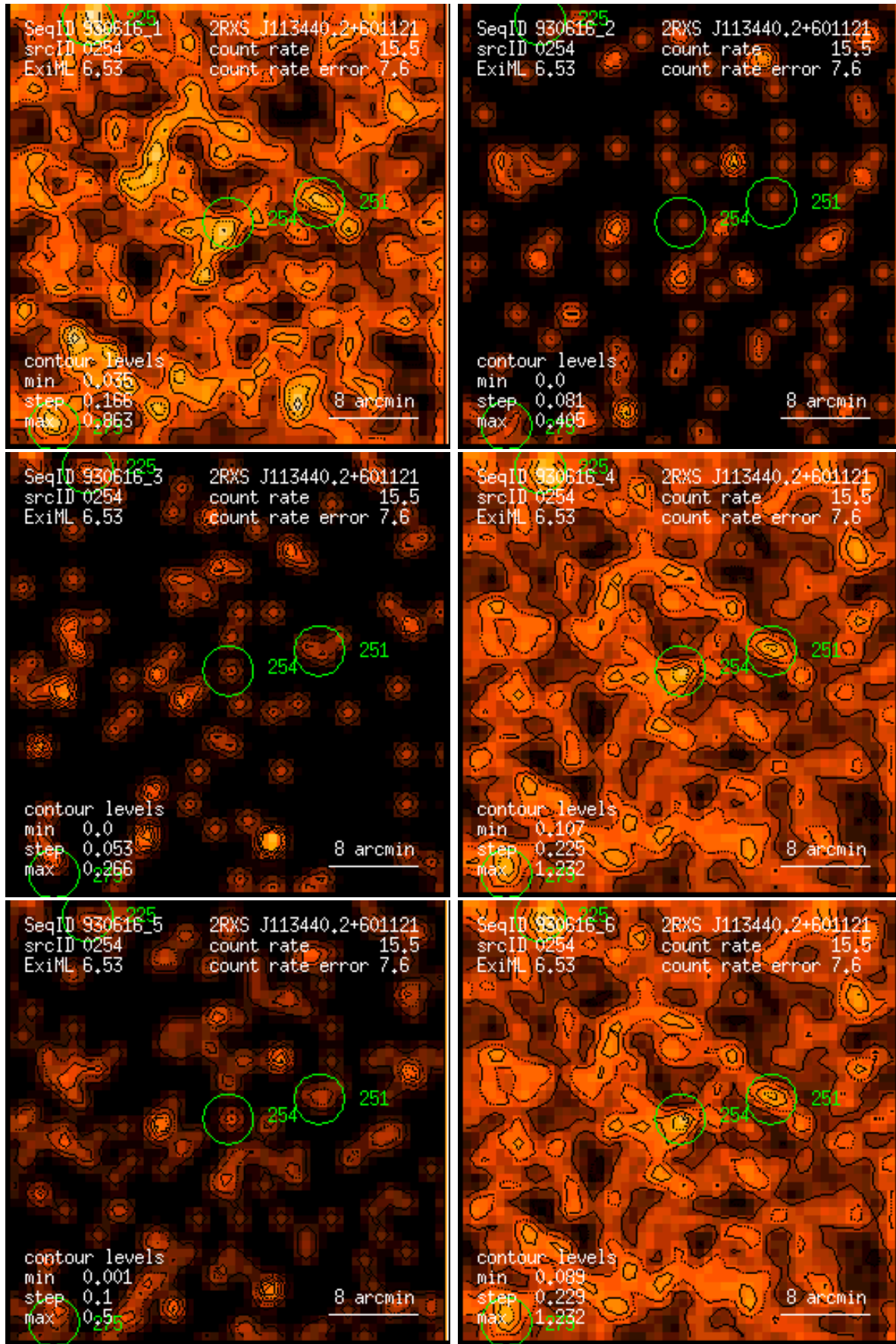
Figure 254: RASS 930616: detection 0254: band rate images, Gaussian filter: (1) PSPC channels 11 – 41, (2) 52 – 90, (3) 91 – 201, (4) 11 – 235, (5) 52 – 201, (6) 11 – 201. Broad band rates in counts/ks. Band rate contour levels in counts/ks/arcmin 2 .
