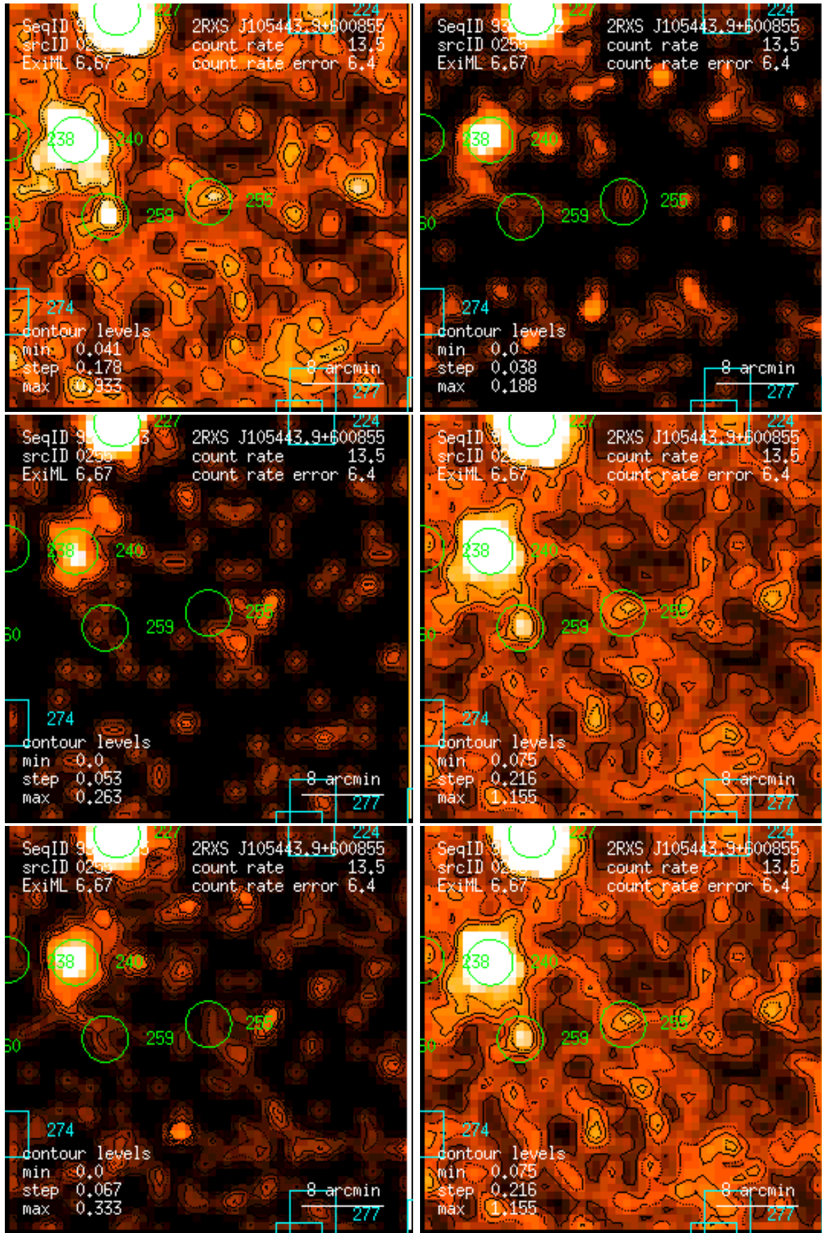
Figure 255: RASS 930616: detection 0255: band rate images, Gaussian filter: (1) PSPC channels 11 – 41, (2) 52 – 90, (3) 91 – 201, (4) 11 – 235, (5) 52 – 201, (6) 11 – 201. Broad band rates in counts/ks. Band rate contour levels in counts/ks/arcmin 2 .
