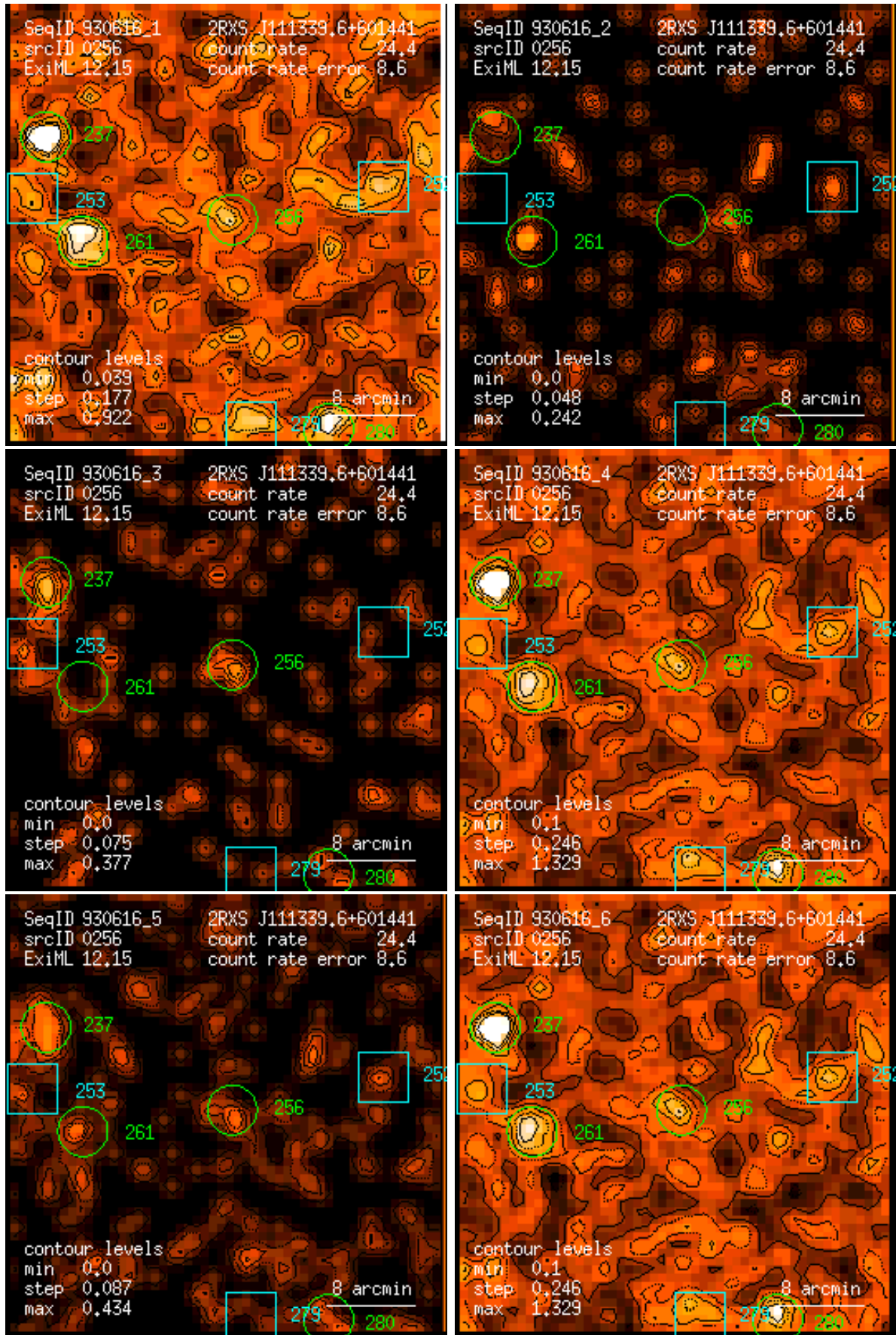
Figure 256: RASS 930616: detection 0256: band rate images, Gaussian filter: (1) PSPPC channels 11 – 41, (2) 52 – 90, (3) 91 – 201, (4) 11 – 235, (5) 52 – 201, (6) 11 – 201. Broad band rates in counts/ks. Band rate contour levels in counts/ks/arcmin 2 .
