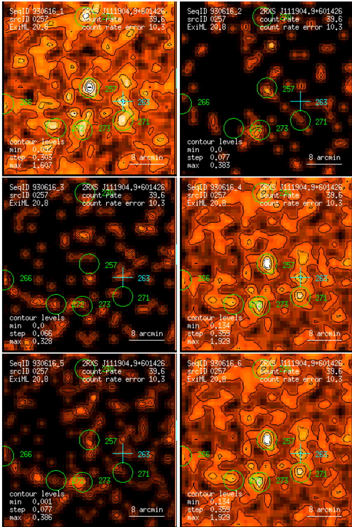
Figure 257: RASS 930616: detection 0257: band rate images, Gaussian filter: (1) PSPC channels 11 – 41, (2) 52 – 90, (3) 91 – 201, (4) 11 – 235, (5) 52 – 201, (6) 11 – 201. Broad band rates in counts/ks. Band rate contour levels in counts/ks/arcmin 2 .
