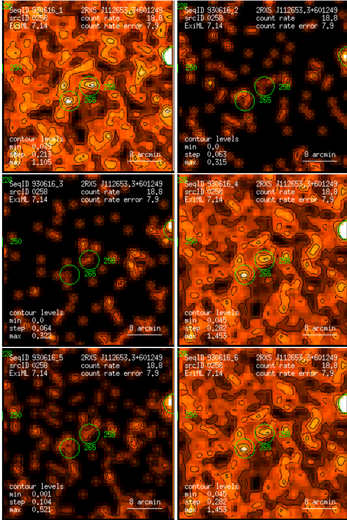
Figure 258: RASS 930616: detection 0258: band rate images, Gaussian filter: (1) PSPC channels 11 – 41, (2) 52 – 90, (3) 91 – 201, (4) 11 – 235, (5) 52 – 201, (6) 11 – 201. Broad band rates in counts/ks. Band rate contour levels in counts/ks/arcmin 2 .
