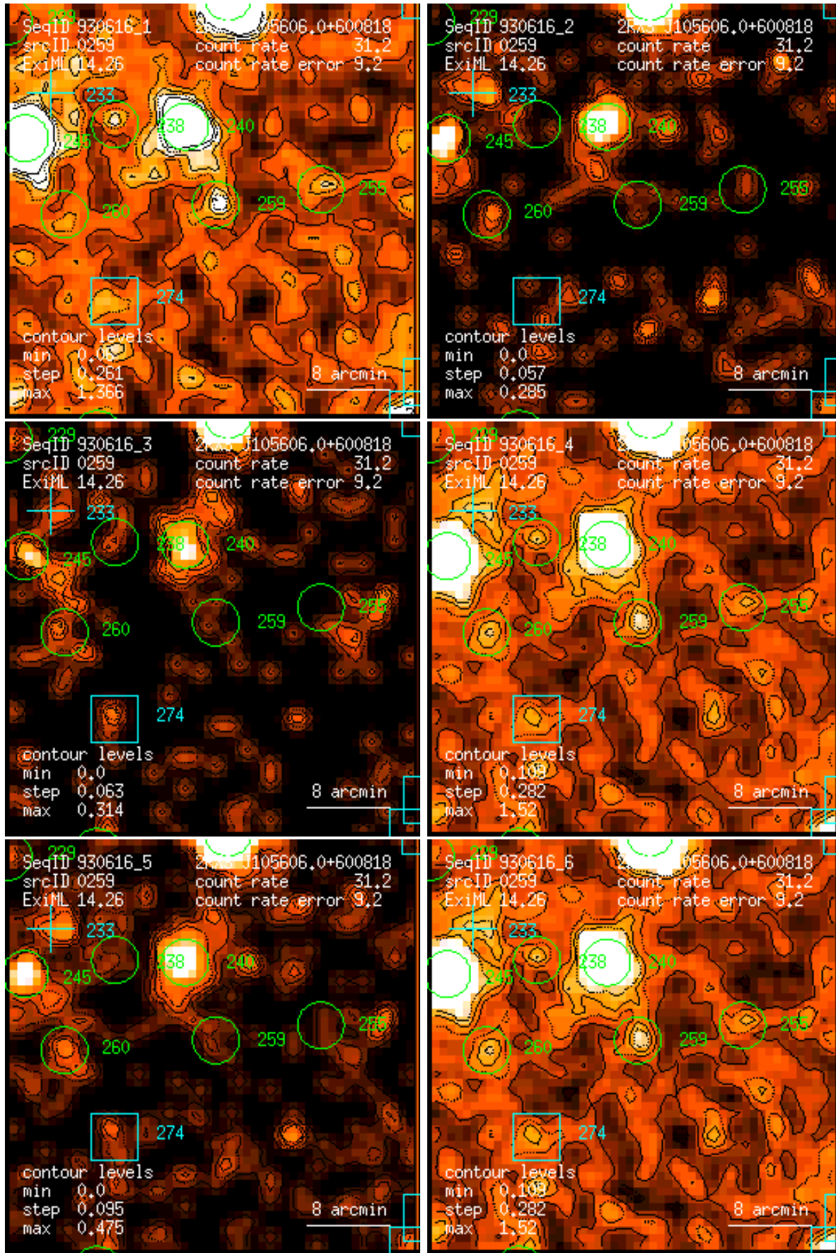
Figure 259: RASS 930616: detection 0259: band rate images, Gaussian filter: (1) PSPC channels 11 – 41, (2) 52 – 90, (3) 91 – 201, (4) 11 – 235, (5) 52 – 201, (6) 11 – 201. Broad band rates in counts/ks. Band rate contour levels in counts/ks/arcmin 2 .
