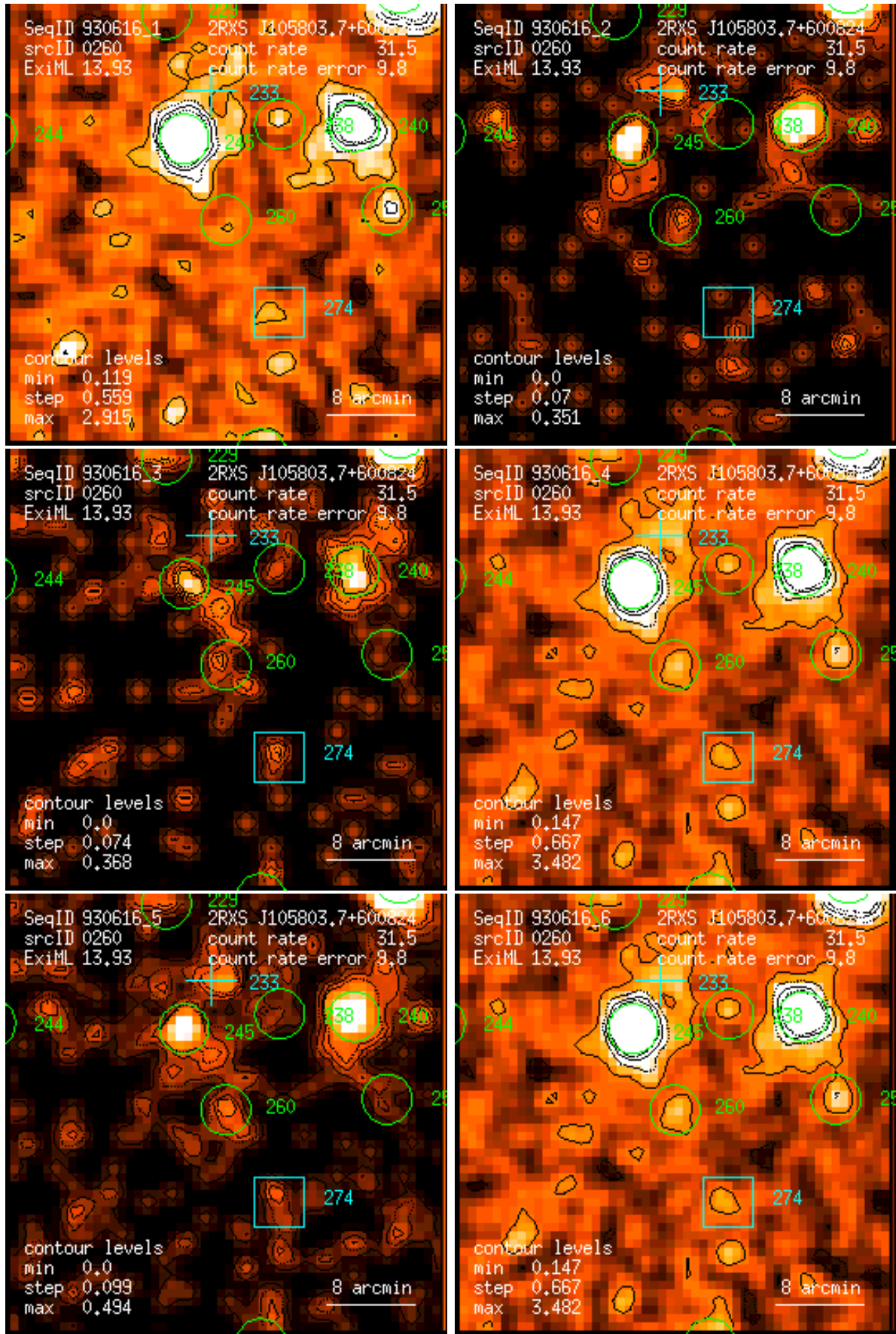
Figure 260: RASS 930616: detection 0260: band rate images, Gaussian filter: (1) PSPC channels 11 – 41, (2) 52 – 90, (3) 91 – 201, (4) 11 – 235, (5) 52 – 201, (6) 11 – 201. Broad band rates in counts/ks. Band rate contour levels in counts/ks/arcmin 2 .
