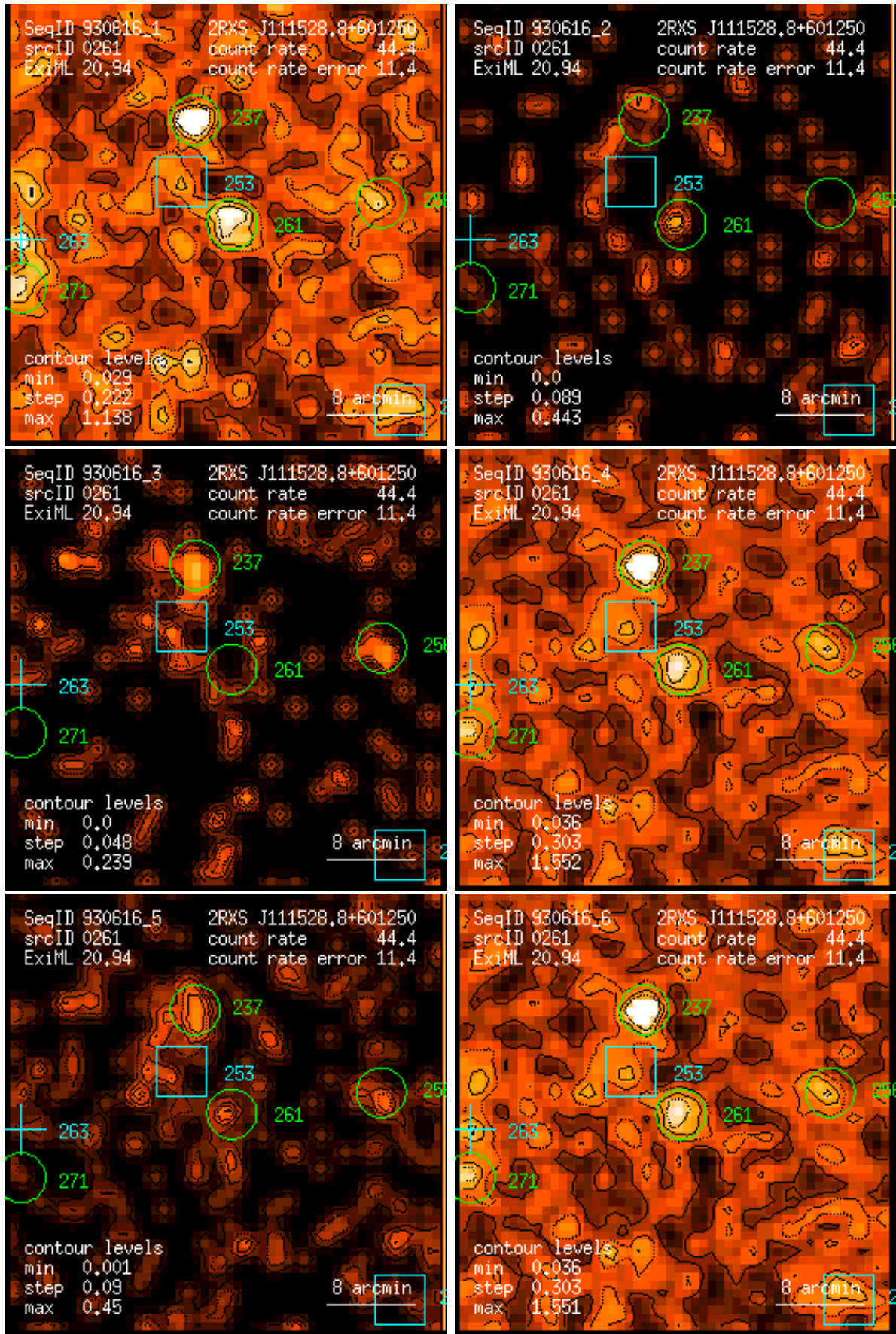
Figure 261: RASS 930616: detection 0261: band rate images, Gaussian filter: (1) PSPC channels 11 – 41, (2) 52 – 90, (3) 91 – 201, (4) 11 – 235, (5) 52 – 201, (6) 11 – 201. Broad band rates in counts/ks. Band rate contour levels in counts/ks/arcmin 2 .
