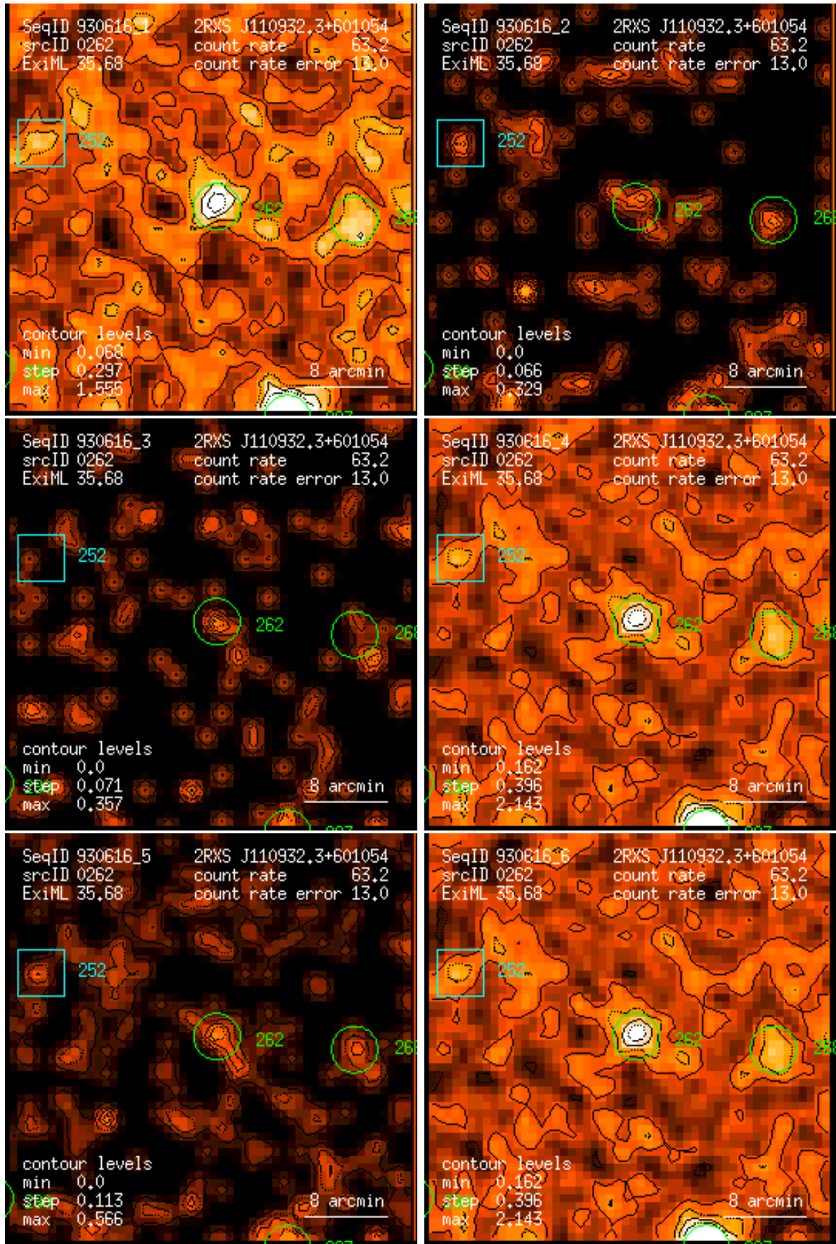
Figure 262: RASS 930616: detection 0262: band rate images, Gaussian filter: (1) PSPC channels 11 – 41, (2) 52 – 90, (3) 91 – 201, (4) 11 – 235, (5) 52 – 201, (6) 11 – 201. Broad band rates in counts/ks. Band rate contour levels in counts/ks/arcmin 2 .
