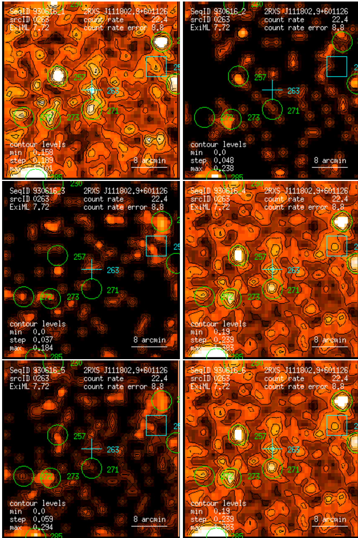
Figure 263: RASS 930616: detection 0263: band rate images, Gaussian filter: (1) PSPC channels 11 – 41, (2) 52 – 90, (3) 91 – 201, (4) 11 – 235, (5) 52 – 201, (6) 11 – 201. Broad band rates in counts/ks. Band rate contour levels in counts/ks/arcmin 2 .
