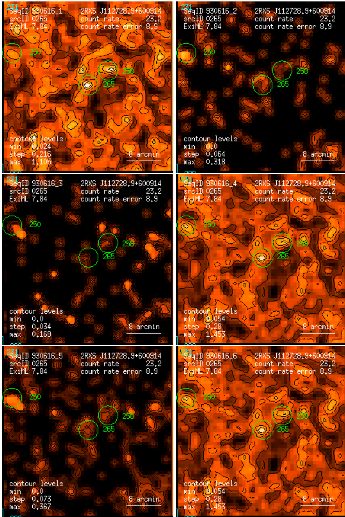
Figure 265: RASS 930616: detection 0265: band rate images, Gaussian filter: (1) PSPC channels 11 – 41, (2) 52 – 90, (3) 91 – 201, (4) 11 – 235, (5) 52 – 201, (6) 11 – 201. Broad band rates in counts/ks. Band rate contour levels in counts/ks/arcmin 2 .
