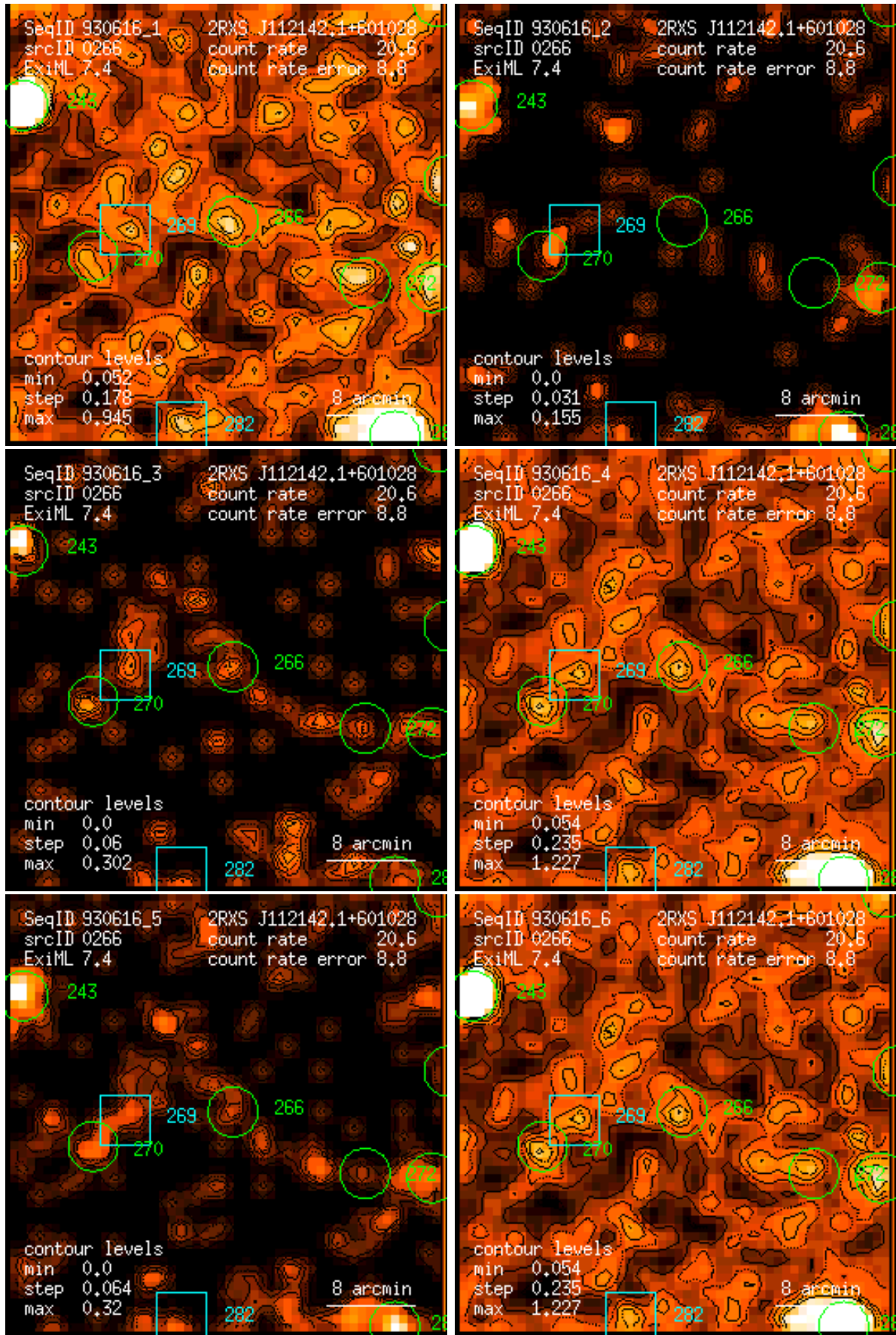
Figure 266: RASS 930616: detection 0266: band rate images, Gaussian filter: (1) PSPC channels 11 – 41, (2) 52 – 90, (3) 91 – 201, (4) 11 – 235, (5) 52 – 201, (6) 11 – 201. Broad band rates in counts/ks. Band rate contour levels in counts/ks/arcmin 2 .
